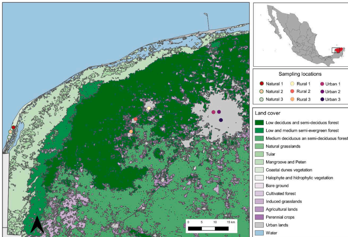
Fig. 1. Distribution of sampling localities along an urbanization gradient (natural, rural, and urban) in the Yucatan state, Mexico. Land cover type is shown according to the National Forest Inventory INEGI-2020.
