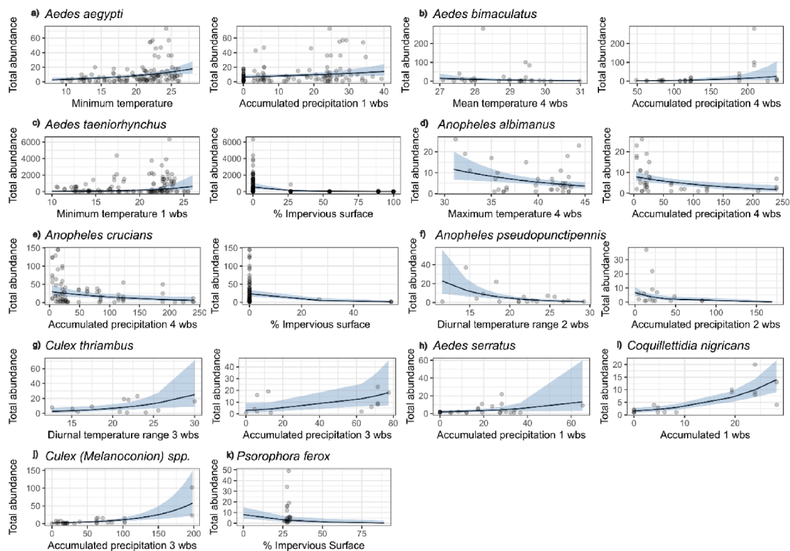
Fig. 5. Results of the generalized linear mixed models, with a negative binomial distribution, showing the effect of the climatic variables and the percentage of impervious surface on the mosquito abundance. Gray points: weekly abundance data, black line: model prediction, and blue area confidence intervals at 95 %.
