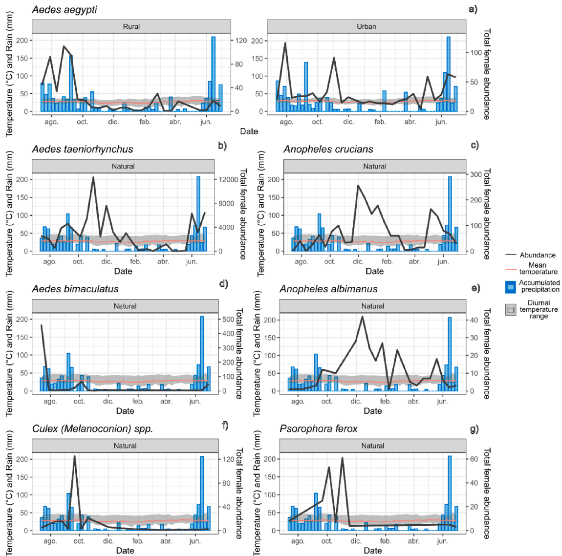
Fig. 4. Annual dynamics of mosquito species in the habitat type in which each species presented the highest abundance (black line: total abundance, blue bars: accumulated precipitation, red line: mean temperature and, gray area: diurnal temperature range). Aedes aegypti was mainly captured in the urban and rural habitats, whereas the other species were mostly captured in natural habitats. The high variation in abundance magnitude is evident on the secondary Y-axis (right side), ranging from 40 individuals captured for An. albimanus to 12,000 individuals captured of Ae. taeniorhynchus .
