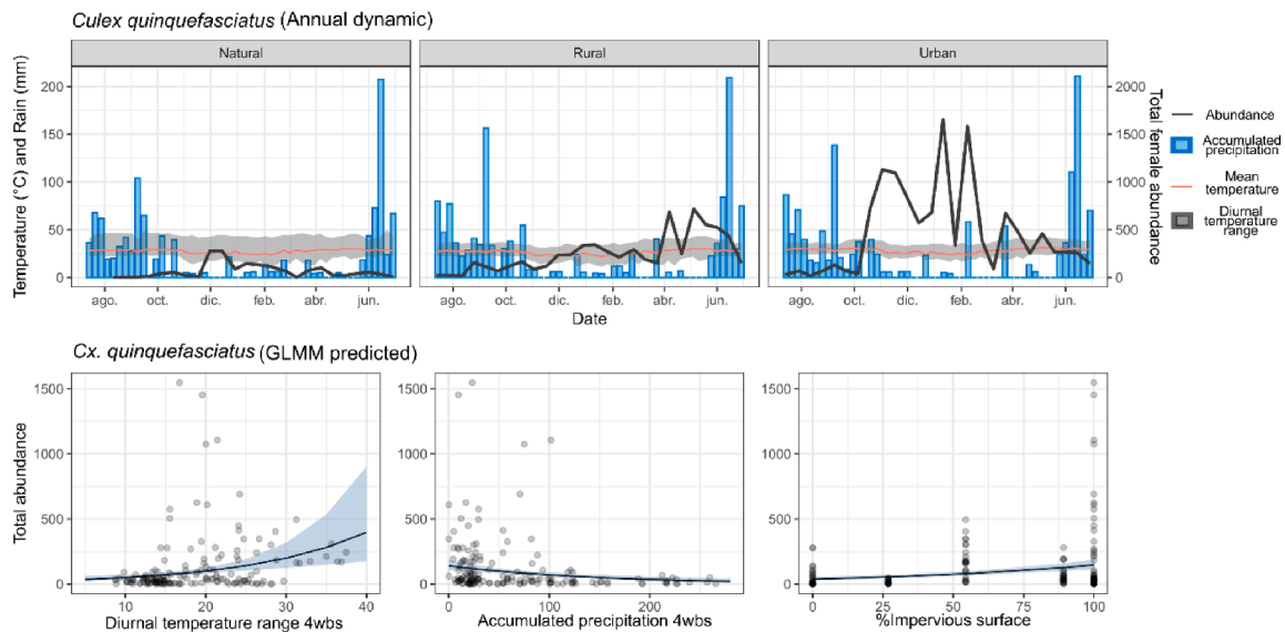
Fig. 3. (a) Annual dynamic of Cx. quinquefasciatus abundance and weekly accumulated climatic variables (black line: total abundance, blue bars: accumulated precipitation, red line: mean temperature and, gray area: diurnal temperature range). (b) Plotted predictions of the generalized linear mixed models showing the effect of the climatic variables and the percentage of impervious surface on the Cx. quinquefasciatus abundance. Gray points: weekly abundance data, black line: model prediction, and blue area confidence intervals at 95%.
