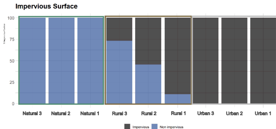
Fig. 2. Land use gradient based on the percentage of impervious surface for each locality (estimated using data National Forest Inventory INEGI-2020).
