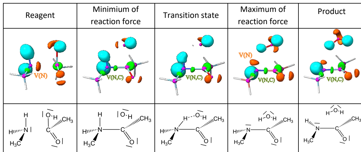
Figure 3: Evolution of the core and valence basins as defined by ELF analysis at the characteristic points of the reaction, for the one-step formation of methylacetamide in the absence of a water molecule, and interpretation in terms of Lewis structures. Basins colored in orange, green and cyan represent monosynaptic V(X) basins, disynaptic V(X,Y) basins, and monosynaptic protonated basins, respectively.
