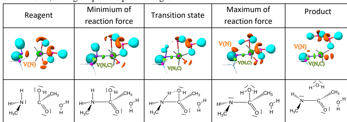
Figure 6: Evolution of the core and valence basins as defined by ELF analysis at the characteristic points of the reaction, for the one-step formation of methylacetamide in the presence of a molecule of water of hydration on acetic acid prior to its reaction, and interpretation in terms of Lewis structures. Basins colored in orange, green and cyan represent monosynaptic V(X) basins, disynaptic V(X,Y) basins, and monosynaptic protonated basins, respectively.
