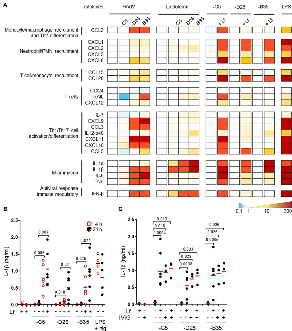
FIGURE 2 | HAdV-lactoferrin complexes induce IL-1α and IL-1β. (A) DCs were incubated with HAdV-C5, -D26, or -B35 ± lactoferrin for 4 h and cytokine secretion in supernatants was assessed by Luminex. To the left of each set of columns is the baseline reference set at zero. For the 4 columns on the left (HAdV), the baseline is mock-infected cells; for the middle columns (Lactoferrin) the baseline reference is lactoferrin-treated cells; for the “paired” columns on the right (-C5, -D26, and -B35) the reference is HAdV-infected cells compared to HAdV-lactoferrin infected cells. Raw data can be found in Figures S2A, B . LPS was used as a control; (B) IL-1β release by DCs in the presence of HAdV-C5, -D26, and -B35 ± lactoferrin was assessed by ELISA at 4 h (red circles) and 24 h (black dots) post-incubation (n = 6, statistical analyses by two-tailed paired t-test). As a control, cells were treated with LPS and nigericin; (C) DCs were incubated with HAdV complexed with lactoferrin, IVIG or lactoferrin + IVIG, for 4 h. IL-1β release was analysed 24 h post-incubation (n ≥ 3, statistical analyses by two-tailed paired t-test).
