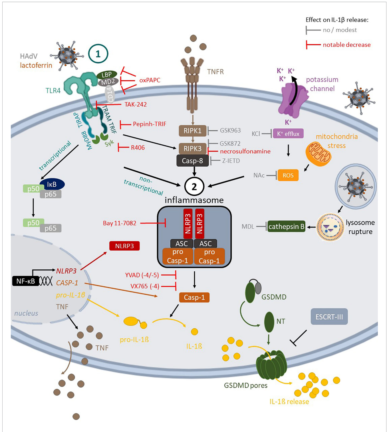
FIGURE 7 | TLR4-mediated HAdV-lactoferrin uptake in DCs and IL-1 \beta release. Lactoferrin binds to HAdV capsid and retargets the capsid toward TLR4 complex on the cells surface. Following TLR4 engagement, its TIR domain recruits MyD88 and TRAM, which bridge TLRs to IRAK and MAPK family members that activate NF- \kappa B, AP-1, and IRF. This priming event initiates transcription of genes coding for inflammasome components (e.g., NLRP3 and IL-1 \beta ). Under prototypic conditions, DCs detect a second perturbation (signal 2) that induced ROS release (mitochondrial stress) or K + efflux (perturbations of cellular integrity), and/or cathepsin B release from lysosome rupture. These pathways do not appear to be activated by HAdV-lactoferrin complexes. In addition to TLR4 pathways, the RIPK1-RIPK3 pathway is activated through an autocrine-TNF release. During inflammasome formation, pro-caspase-1 auto-activation induces cleavage of pro-IL-1 \beta and likely GSDMD, which will initiate, but not complete, the loss of plasma membrane integrity via pore formation, allowing IL-1 \beta release. Twenty-four hours post-challenge, DC membrane integrity is intact, consistent with the involvement of ESCRT-III complex and repairing GSDMD pores.
