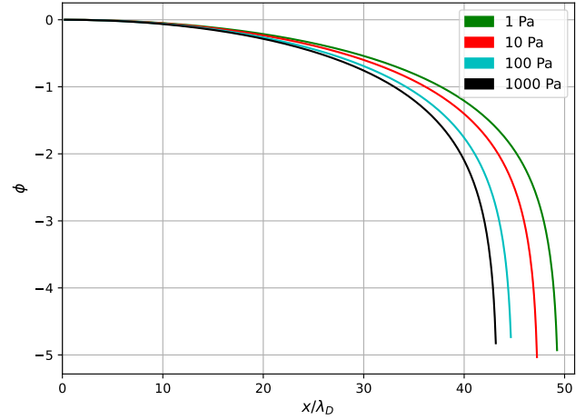
Figure 3: Analytical profile of the electric potential obtained with eq.(14) at different background pressures ( green : 1 Pa, red : 10 Pa, cyan : 100 Pa, black : 1000 Pa).
