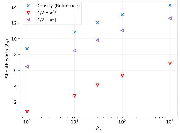
Figure 11: Estimations of the sheath width for different background pressures width using three different approaches to obtain the sheath edge position: the position where the charge density for DD results equals \bar{\rho}_C = 0.049 ("Density (Reference)", eq.(17) and eq.(19) with \bar{\rho}_C = 0.049 . x^{As} and x^\rho are computed using the ionization frequency from the drift-diffusion simulations.
