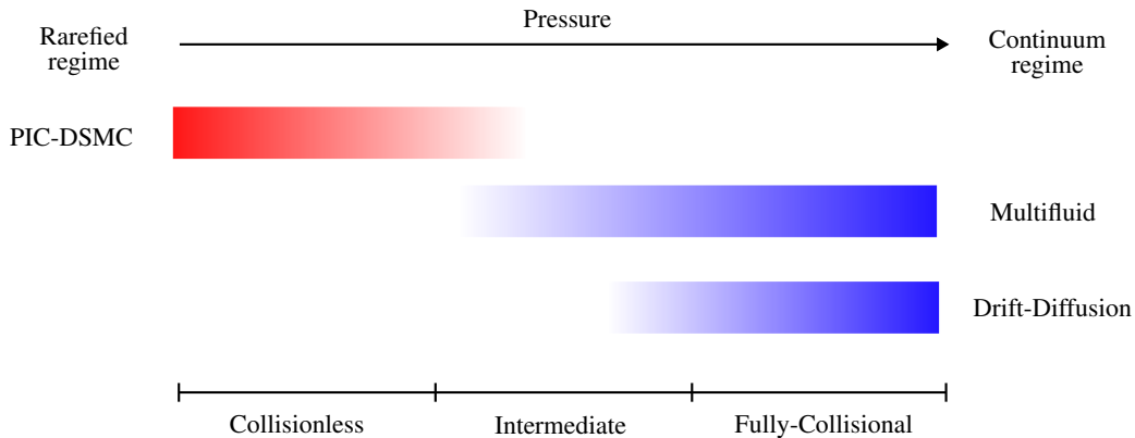
Figure 1: Qualitative scheme representing the range of applicability of different numerical methods for plasma physics. The gas pressure, increasing from the rarefied to the continuum regime, defines three conditions: collisionless, intermediate and fully-collisional. Red : particle-method, blue : fluid models.
