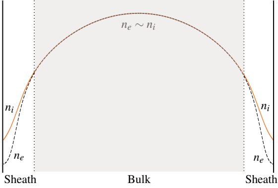
Figure 2: Schematic of the one-dimensional discharge.
