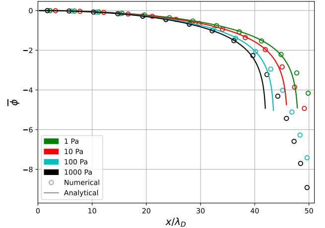
Figure 12: Comparison of analytical profiles ( solid ) of the electric potential \bar{\phi} = \phi/\phi_0 , obtained with eq.(15) with numerical solutions ( circles ), at different background pressures.
