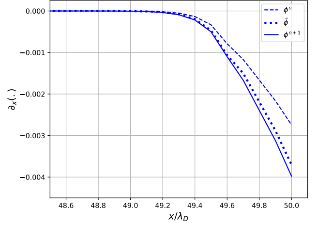
Figure 4: Gradient of the electric potential \phi evaluated at timestep n (dashed), n+1 (full) and the predicted value obtained with eq.(22) (dots). Values obtained at the first steps of the simulation.
