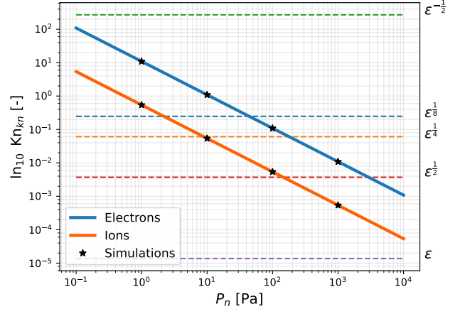
Figure 5: Knudsen number for electrons ( blue ) and ions ( orange ) at different background gas pressures, with order of magnitudes highlighted in terms of powers of the mass ratio \varepsilon . The lengthscale L_0 = L is the width of the domain, the characteristic length of the bulk. Simulation conditions are shown ( stars ).
