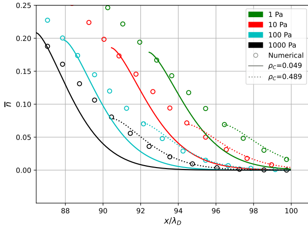
(b) Electron number density.
