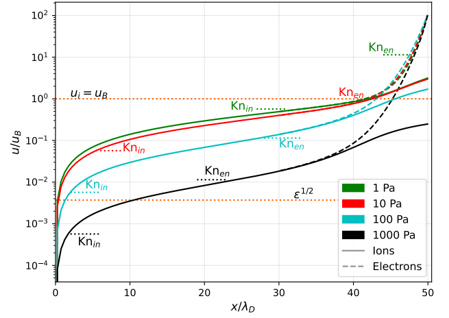
Figure 9: Electrons (dashed) and ions (solid line) velocity obtained with multifluid simulations varying the background gas pressure ( green : 1 Pa, red : 10 Pa, cyan : 100 Pa, black : 1000 Pa). Orders of magnitude are highlighted with dotted lines compared to the mass ratio \epsilon , the collisionless Bohm velocity u_B and Knudsen numbers Kn_{en} and Kn_{in} .
