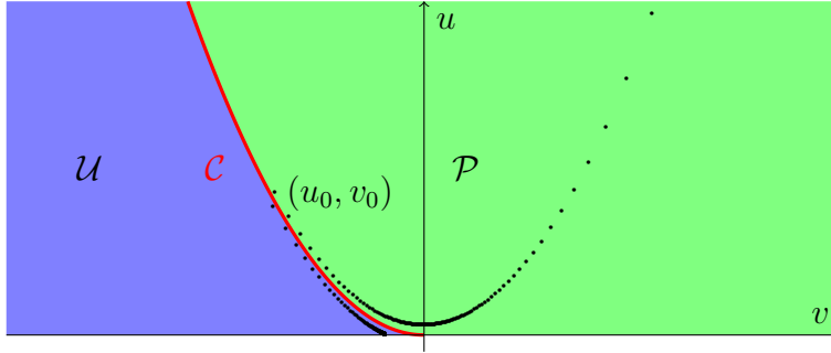
FIGURE 1. Decomposition of the phase space for a function \Psi defined by \Psi(x) = x^2/2(1+x-\sqrt{1+2x}) for x \in [-0.5, 0.5] , extended to \mathbb{R} in such a way that (A) holds. For this function, the critical curve h is given by x \mapsto x^2/2 on [-0.5, 0.5] and drawn in red. Additionally, slightly supercritical and subcritical trajectories for (u, v) are depicted.
