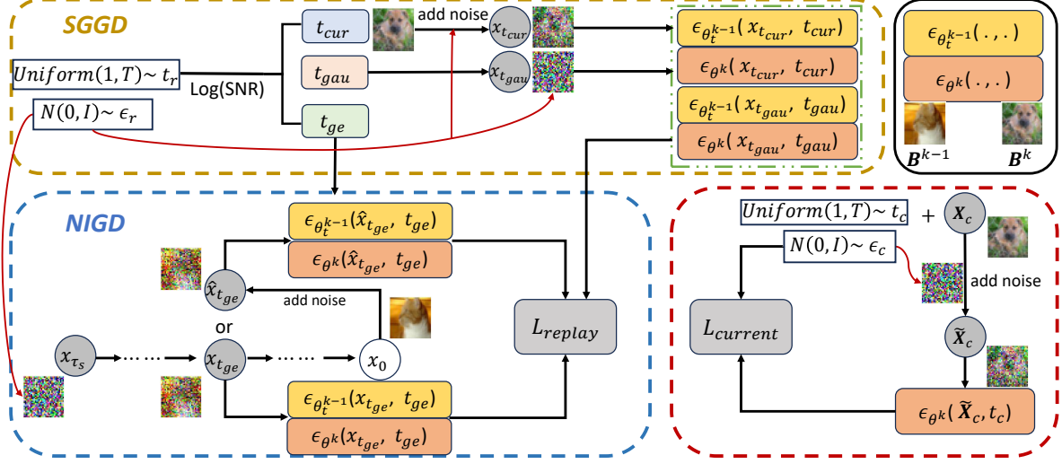
Fig. 1. Illustration of Our Method. The yellow region represents SGGD, the blue region denotes NIGD, and the red region corresponds to training on the current batch \mathbb{B}^k . \epsilon_{\theta_{tea}^{k-1}} is our EMA-teacher, and \epsilon_{\theta^k} is our current model.
