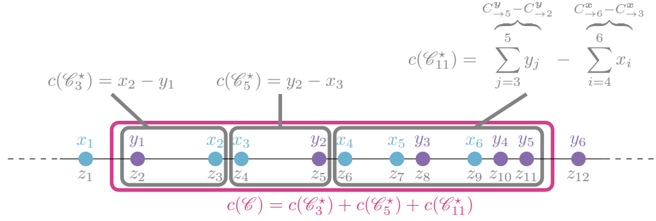
Figure 2: Chains and their associated costs. In order to compute the cost for chain \mathcal{C} (in magenta), we partition it into a sequence of 3 minimal chains \mathcal{C}_3^* , \mathcal{C}_5^* and \mathcal{C}_{11}^* , for which cost computation can be made efficient when the Manhattan distance is considered.
