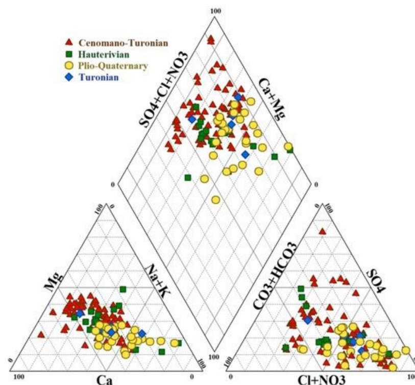
Figure 13. Piper diagram of the analyzed samples (campaign of 2020).
