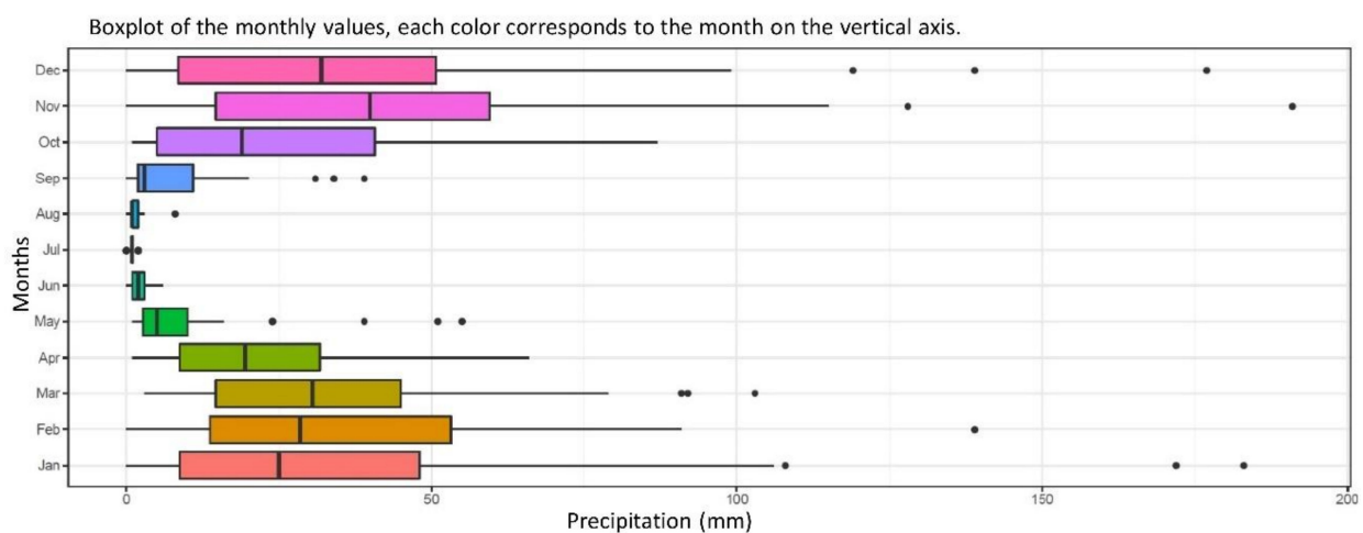
Figure 5. Boxplot of monthly values between 1979 and 2019.
