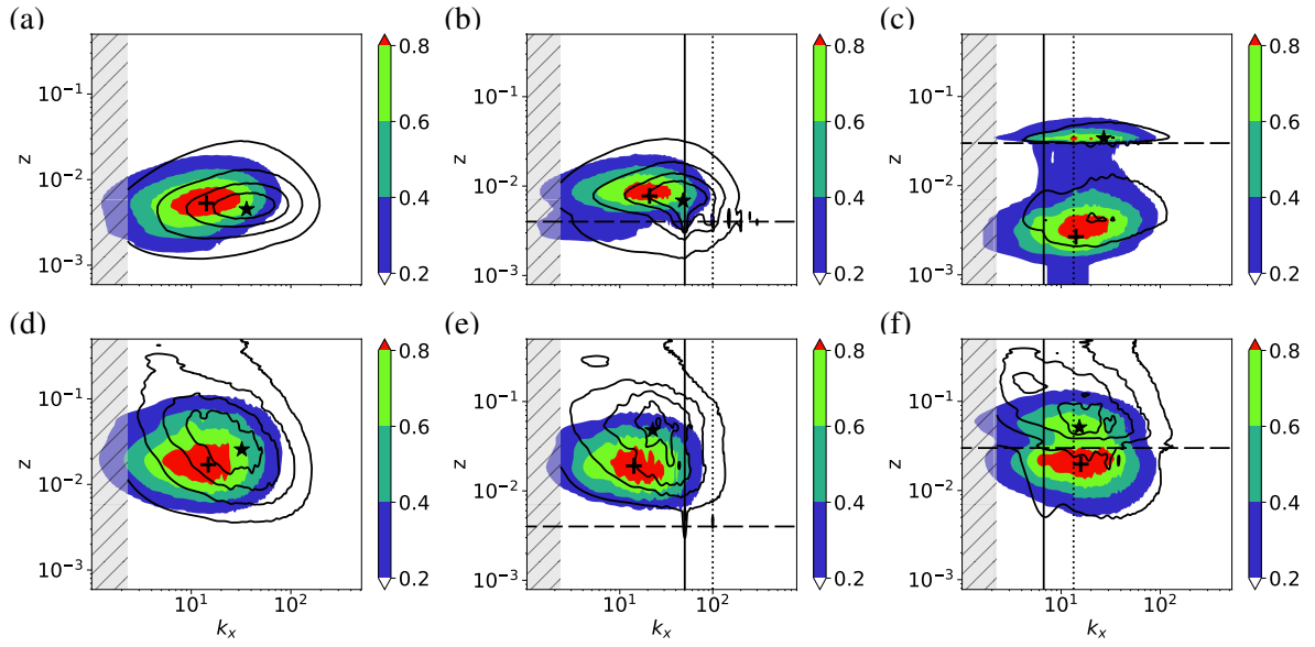
Figure 2: The premultiplied temperature power spectrum k_x E_{\theta'\theta'} (top) and the premultiplied heat flux co-spectrum k_x E_{w'\theta'} (bottom) normalized by the maximum density value of each case, where k_x is the wavenumber in the horizontal direction e_x and computed in the bottom half of the domain at y = \Gamma_y/2 . The three geometrical configurations are displayed: (left) SS cases; (middle) RS2 cases; (right) RS3 cases. Colours correspond to the cavity cases and lines to the periodic configurations. The grey shaded areas correspond to the unreachable k_x in the periodic configurations because of the reduced size of the domain. The solid (resp. dashed and dotted) line corresponds to k_p = 1/\lambda_p (resp. h_p and k_v = 1/w_v ). Marker + (resp. \star ) points to the peak location of the spectral density in the cavity (resp. in periodic configurations).
