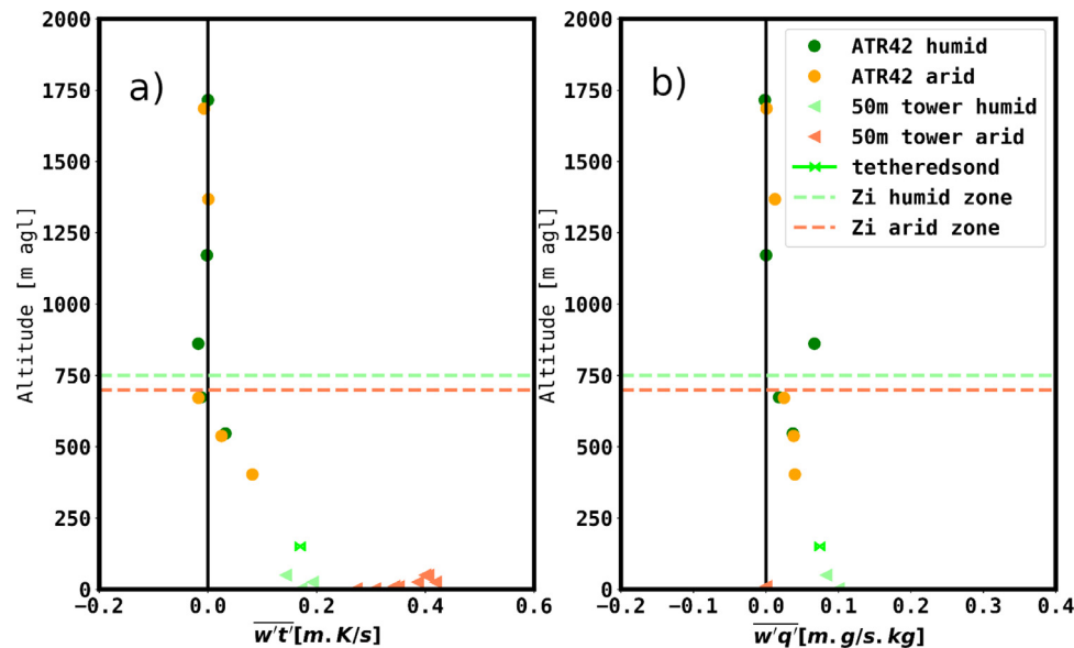
Fig. 5. Vertical profile of kinematic (a) heat flux and (b) moisture flux observed on July 15 2021. Orange and green symbols denote the two different explored areas, arid (rained) and humid (irrigated), respectively. Dashed lines represent the ABL top ( Z_i ).
