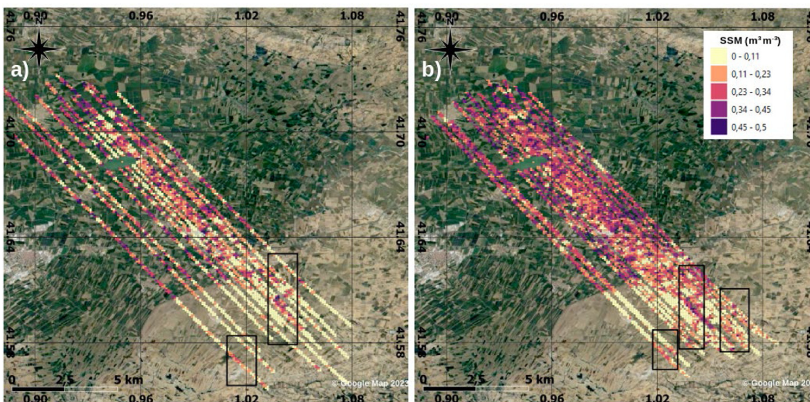
Fig. 6. SSM maps (100 m spatial resolution) retrieved from the \Gamma_{RL} (reflectivity) inversion: (a) Flight 45 on 22 July 2021 during dry conditions, (b) Flight 46 on 27 July 2021 which was relatively wetter after a precipitation event. The boxes indicate zones containing fields with drip irrigation (pixels with relatively larger SSM) which were not seen by disaggregated SSM products. The background map is from Google Map (last accessed in 2023).
