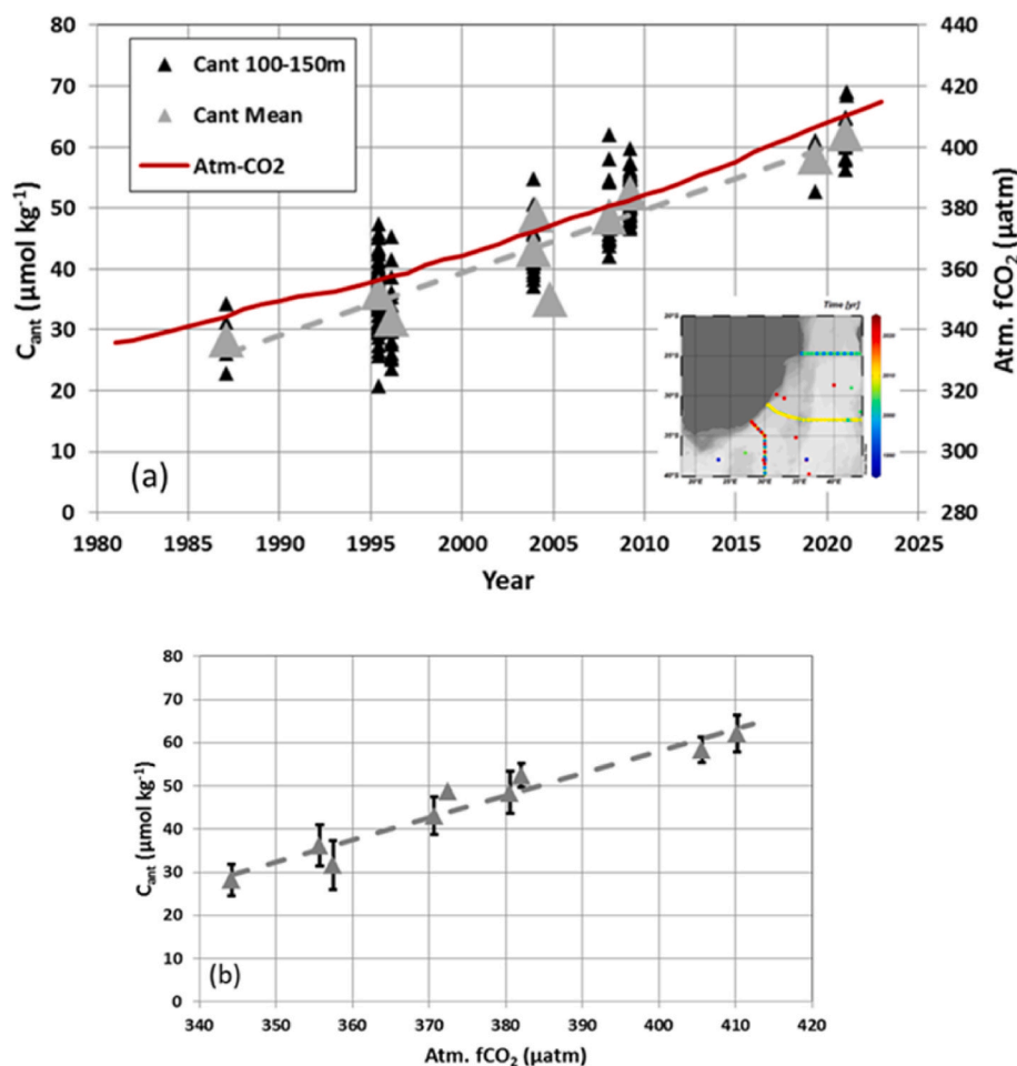
Fig. 7. (a) Time-series of anthropogenic CO_2 concentrations ( C_{ant} ) over 1987–2021 estimated in subsurface (layer 100–150m) from the GLODAP-v2023 data (Lauvset et al., 2024) completed with OISO cruise in 2021 (location of selected stations in the insert map, color code is for year). The figure shows the C_{ant} concentrations calculated for each sample (black) and the C_{ant} averaged in the layer 100–150m for each period (grey triangles). Over the period 1987–2021, the C_{ant} trend is +1.03 \pm 0.14 \mu mol kg^{-1} yr^{-1} (dashed grey line). The red curve is the atmospheric fCO_2 . (b): same data for C_{ant} versus atmospheric fCO_2 (slope = +0.512 \pm 0.050 \mu mol kg^{-1} \mu atm^{-1} ).
