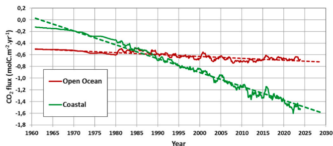
Fig. 10. Reconstructed time-series of the CO 2 fluxes (molC.m -2 .yr -1 ) in the Mozambique Basin (open ocean region, red) and in the African coastal zone (green). Corresponding linear trends are indicated in dashed.
