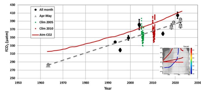
Fig. 6. Time-series of monthly mean fCO_2 ( \mu atm , black dots for all season and grey triangles for April–May) in the Mozambique Basin (region 24^\circ S-35^\circ S/32^\circ E-42^\circ E ). The red curve is the atmospheric fCO_2 . The monthly climatology for a reference year 2005 or 2010 (Takahashi et al., 2014; Fay et al., 2024) is also plotted (green and red diamonds) highlighting the seasonality in this region. For the period April–May the oceanic fCO_2 increase of +1.79 \pm 0.13 \mu atm.yr^{-1} (dashed grey line) is close to the atmospheric increase. The selected tracks in April–May are indicated in the insert map produced with ODV (Schlitzer, 2018). The mean monthly values and standard deviations are listed in Table 2.
