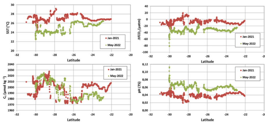
Fig. 3. Distribution of sea surface temperature, \Delta fCO_2 , C_T , and pH in January 2021 (red) and in May 2022 (green) along the same track in the southwestern Indian Ocean (from La Réunion to Durban). Average values are listed in Table 1.
