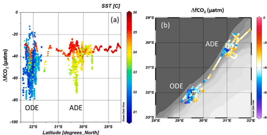
Fig. 4. Distribution of \Delta fCO_2 ( \mu atm ) during the RESILIENCE cruise in May 2022 along the African coast. In (a) color code is for SST (°C). In (b) color code is for \Delta fCO_2 ( \mu atm ). “ADE” and “ODE” identifies the locations of the Active Durban Eddy and the Old Durban Eddy investigated during the cruise. In May 2022, the ocean was always a CO_2 sink in this region ( \Delta fCO_2 < 0 ). Figures produced with ODV (Schlitzer, 2018).
