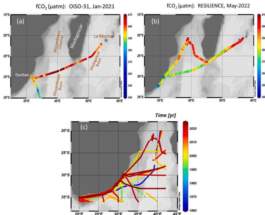
Fig. 1. Maps of OISO-31 cruise (a) and RESILIENCE cruise (b) conducted in January 2021 and April–May 2022; color code is for sea surface fCO 2 (µatm). (c) Tracks of cruises in the SOCAT data-base, v2024 (Bakker et al., 2016, 2024); color code is for Year (1963–2023). Figures produced with ODV (Schlitzer, 2018).
