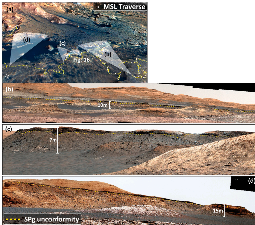
Fig. 14. Exposure of the SPg unconformity along the northern and eastern margin of the Greenheugh pediment. a) Mastcam location and look angles for Mastcam mosaics in b-d. b) Northern margin of the pediment. c) Northeast margin of the pediment. d) Eastern extent of the pediment escarpment south of Siccar point showing planar SPg unconformity and patches of regolith mantle flanking the escarpment. HiRISE image credit: NASA/JPL/University of Arizona. Mastcam image credit: NASA/JPL-Caltech/MSSS. See Table S1 in Supporting information S3 for image sequence identifiers.
