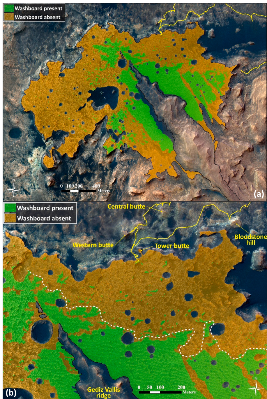
Fig. 7. Washboard pattern mapped from HiRISE orthoimagery showing areas of ‘intact’ washboard (green) and areas of non-washboard Stimson (orange). a) full pediment map. b) Inset showing the NE pediment area including the approximate boundary (white dashed line) between coherent washboard and the lower Stimson units. HiRISE image credit: NASA/JPL/University of Arizona. (For interpretation of the references to colour in this figure legend, the reader is referred to the web version of this article.)
