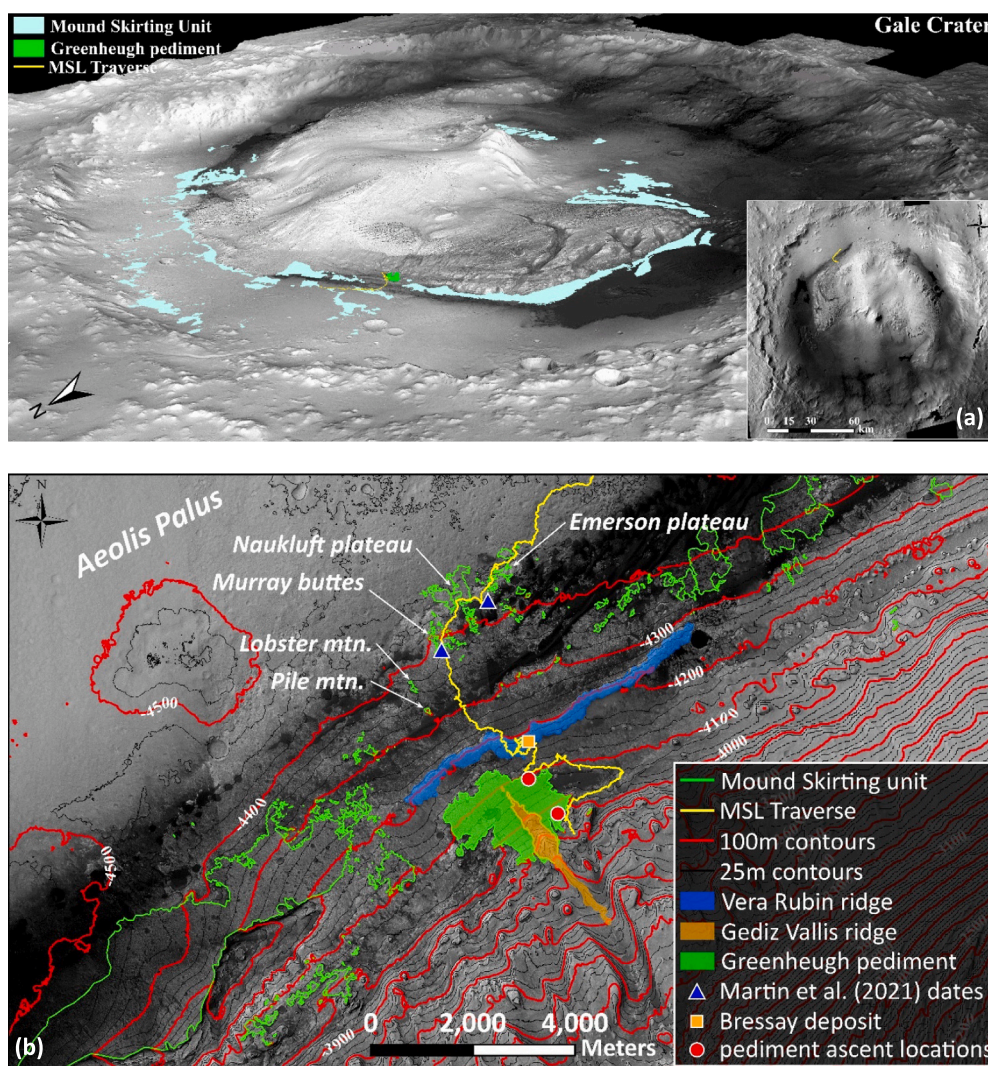
Fig. 1. Context maps of Gale crater and northern Mt. Sharp. a) 3D and map (inset) view of Gale crater made using imagery from the Context Camera (CTX) instrument on board the Mars Reconnaissance Orbiter (MRO) (Malin et al., 2007). The Greenheugh pediment is highlighted in green along with Curiosity's traverse (yellow) and the Mound skirting unit (teal) mapped by Anderson and Bell (2010) (light blue). b) Map of the northern footslopes of Mt. Sharp showing 25 (black) and 100 (red) meter HiRISE contours on a shaded relief image. Data from: McEwen et al. (2007), Calef III and Parker (2016), and Parker and Calef III (2016). The Greenheugh pediment is shown shaded in green, Vera Rubin ridge in blue, and the Gediz Vallis ridge in orange. Outline in green is a compilation of our own orbital mapping as well as: Mound Skirting unit features south of Aeolis Palus mapped by Anderson and Bell (2010) and Siccar Point group features mapped by Fraeman et al. (2016); Stack et al. (2017); Kronyak et al. (2019); Watkins et al. (2022); Banham et al. (2018); Banham et al. (2022). Pediment ascent locations, the Bressay heterolithic deposit as well as locations for radiometric exposure a (Martin et al., 2021) are also indicated on the map along the MSL traverse (yellow). HiRISE image credit: NASA/JPL/University of Arizona. (For interpretation of the references to colour in this figure legend, the reader is referred to the web version of this article.)
