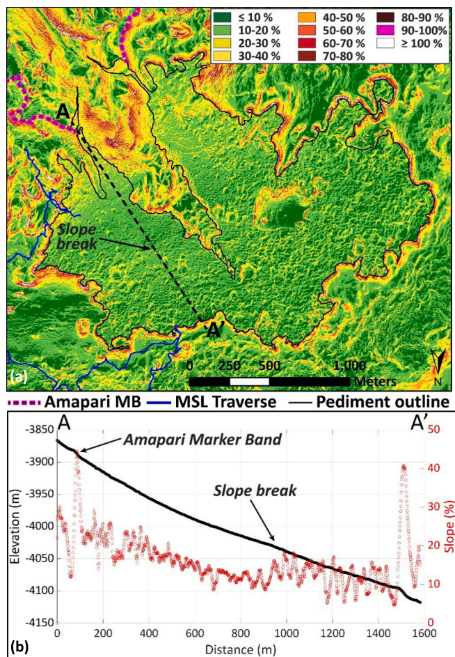
Fig. 6. Slope map and associated long-profile at the Greenheugh pediment. a) Slope map from HiRISE-derived topography with the Amapari Marker Band (MB) overlain in purple and the MSL traverse in blue. b) Elevation and slope profile A-A' taken from the SE side of the pediment perpendicular to topography. Note in the profile the locations of slope anomalies at the Northern edge of the pediment, near the center of the profile (labeled slope break) and at the Amapari Marker Band (Purple dashed line in (a) (Milliken et al., 2010; Weitz et al., 2022)). HiRISE image and topographic data source credit: NASA/JPL/University of Arizona. (For interpretation of the references to colour in this figure legend, the reader is referred to the web version of this article.)
