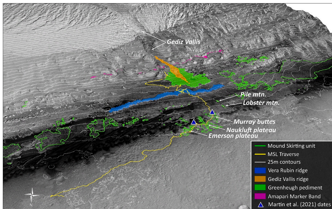
Fig. 2. Footslope of Mt. Sharp looking towards the south. The Greenheugh pediment is shown shaded in green, Vera Rubin ridge in blue, and the Gediz Vallis ridge in orange. Outline in green is a compilation of our own orbital mapping as well as: Mound Skirting unit features south of Aeolis Palus mapped by Anderson and Bell (2010) and Siccar Point group features mapped by Fraeman et al. (2016); Stack et al. (2017); Kronyak et al. (2019); Watkins et al. (2022); Banham et al. (2018); Banham et al. (2022). The Amapari Marker Band (Milliken et al., 2010; Weitz et al., 2022) is shown (purple) as well as locations for radiometric exposure ages (Martin et al., 2021) are also indicated on the map along the MSL traverse (yellow). HiRISE image credit: NASA/JPL/University of Arizona. HiRISE image credit: NASA/JPL/University of Arizona. (For interpretation of the references to colour in this figure legend, the reader is referred to the web version of this article.)
