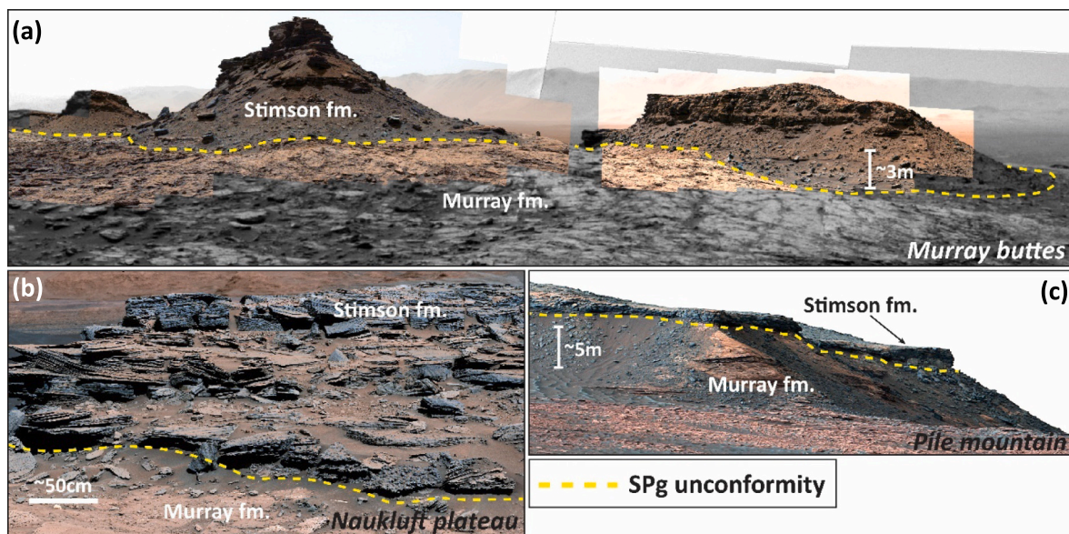
Fig. 4. Mastcam images showing areas exposures to the north (and downslope from) the Greenheugh pediment. Locations for a) Murray buttes, b) Naukluft plateau, c) Pile mountain are shown in Figs. 1b and 2. The basal Siccar Point group (SPg) unconformity (yellow dashed line) separates the Stimson formation (SPg) from the Murray formation within the Mt. Sharp group (MSg). Image credit: NASA/JPL-Caltech/MSSS. See Table S1 in Supporting information S3 for image sequence identifiers. (For interpretation of the references to colour in this figure legend, the reader is referred to the web version of this article.)
