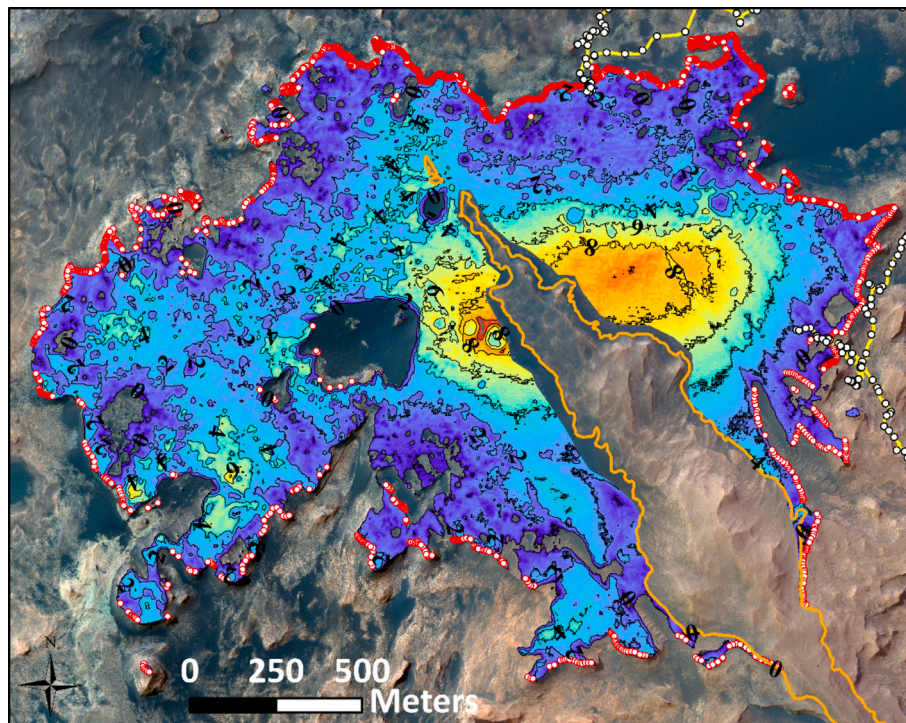
Fig. 21. Contoured thickness map of the Stimson formation on the Greenheugh pediment. Red dots indicate locations where the SPg unconformity could be reliably identified due to both a topographic inflection and a change in HiRISE false colour image tone. Locations were confirmed with Mastcam where possible. Thicknesses in the interior pediment was derived from a thin plate approximation. HiRISE image credit: NASA/JPL/University of Arizona. (For interpretation of the references to colour in this figure legend, the reader is referred to the web version of this article.)
