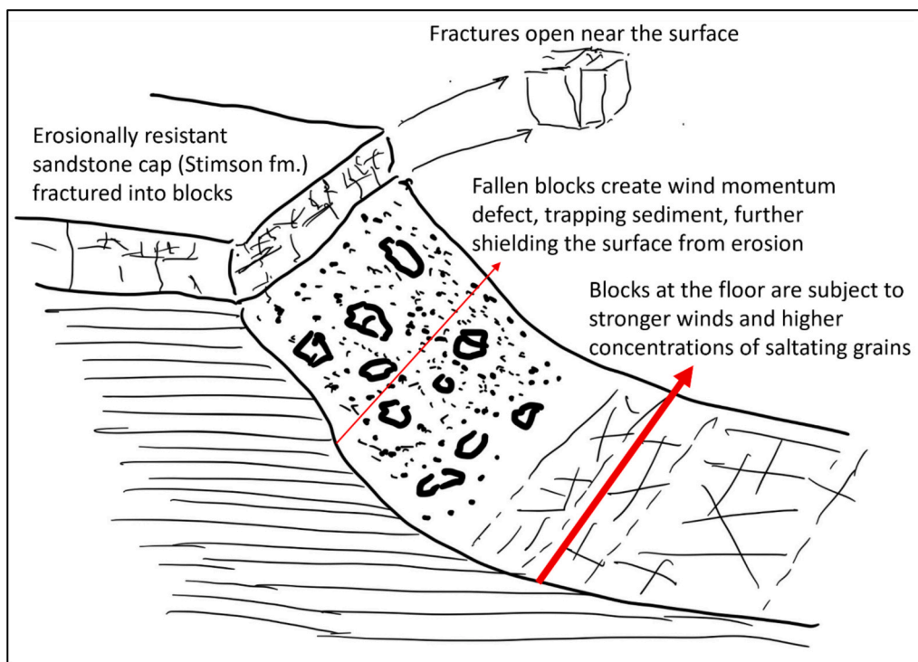
Fig. 27. Schematic diagram showing relationship between fallen Stimson boulders and local sand accumulation characteristic of the steep side slopes flanking many of the buttes observed by Curiosity. Boulder and associated sand mantling retard scarp retreat. Enhanced wind abrasion removes blocks at the base of retreating buttes.
