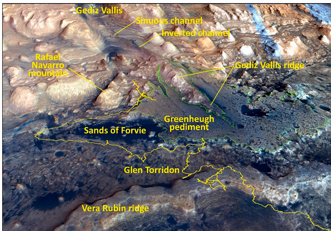
Fig. 3. View of footslope looking towards the south. The MSL traverse (yellow) onto and around the Greenheugh pediment (green outline) is also included. HiRISE image credit: NASA/JPL/University of Arizona. (For interpretation of the references to colour in this figure legend, the reader is referred to the web version of this article.)
