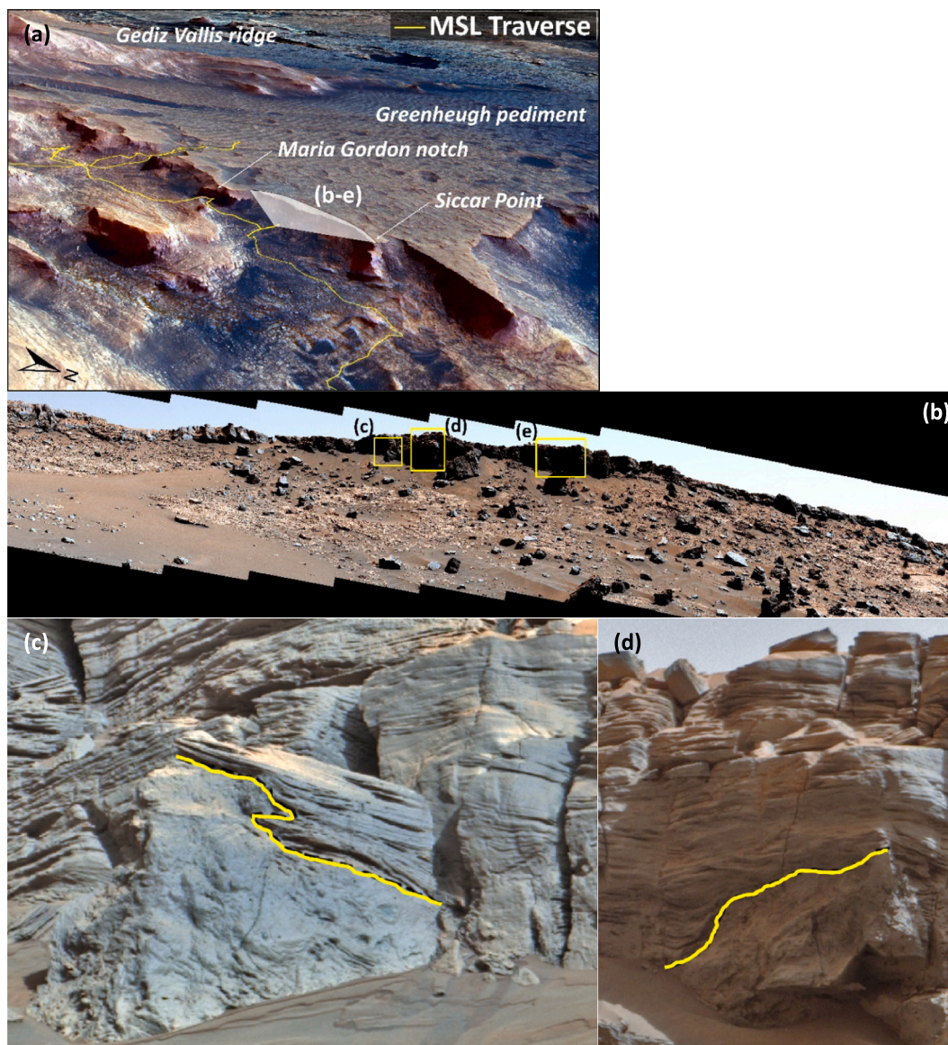
Fig. 16. Pediment escarpment exposure revealing soft sediment deformation features in the lower Stimson. a) 3D view of the outcrop exposure located between Siccar Point and Maria Gordon notch. (b-e) Mastcam mosaics of the basal Stimson (b) showing loss of coherent bedding, as well as the irregular boundary between the deformed sediments and the undisturbed upper layers including evidence for possible fluid escape paths. (f-h) Mastcam mosaics of tumbled blocks accessed for chemical analysis and grain size measurements. HiRISE image credit: NASA/JPL/University of Arizona. Mastcam image credit: NASA/JPL-Caltech/MSSS. See Table S1 in Supporting information S3 for image sequence identifiers.
