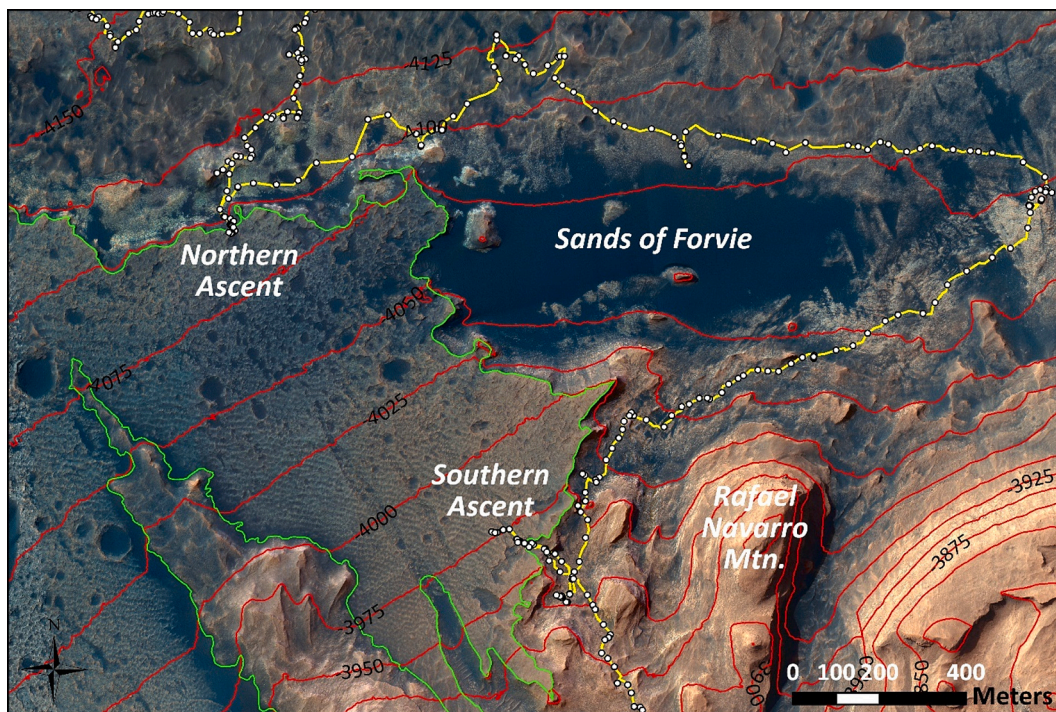
Fig. 8. Map of the eastern side of the Greenheugh pediment showing the two ascent locations northern (Tower butte) and southern (Blackcraig) as well as the MSL traverse around the Sands of Forvie. HiRISE image credit: NASA/JPL/University of Arizona.
