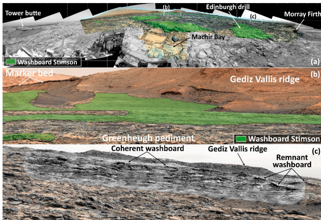
Fig. 13. Top surface of the Stimson-mantled Greenheugh pediment looking south towards Mt. Sharp. a) Green area indicates pieces of preserved washboard structure. b) Boundary between preserved washboard surface near the Gediz Vallis ridge and degraded Stimson (no colour). c) Inset from (a) showing Mastcam and ChemCam RMI imagery of the distal Gediz Vallis ridge as well as areas of coherent and remnant washboard below. Image credit: NASA/JPL-Caltech/MSSS. See Table S1 in Supporting information S3 for image sequence identifiers. (For interpretation of the references to colour in this figure legend, the reader is referred to the web version of this article.)
