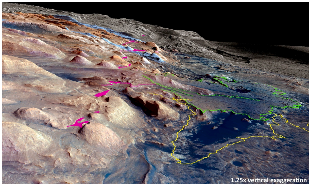
Fig. 25. A 3D HiRISE view of the NW margin of Mt. Sharp facing WSW including the Greenheugh pediment (green outline), Amapari Marker Band (purple), and Curiosity's traverse (yellow). Note the 1.25 \times vertical exaggeration. HiRISE image credit: NASA/JPL/University of Arizona. (For interpretation of the references to colour in this figure legend, the reader is referred to the web version of this article.)
