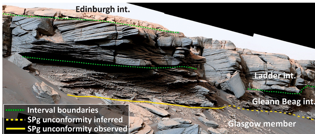
Fig. 12. Greenheugh pediment showing the SPg unconformity and Stimson stratigraphic intervals (“int.”) as defined by Banham et al. (2022). Image credit: NASA/JPL-Caltech/MSSS. See Table S1 in Supporting information S3 for image sequence identifiers. Note the Stimson cliff in this image is ~1.5 m thick.
