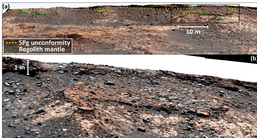
Fig. 15. Pediment exposure west of Bloodstone hill (see Fig. 14a for look angle). a) Residual scree slope mantle (green dashed lines) along the pediment margin that suggest episodic or differential scarp retreat. b) A closer view of the mantle patch Image credit: NASA/JPL-Caltech/MSSS. See Table S1 in Supporting information S3 for image sequence identifiers. (For interpretation of the references to colour in this figure legend, the reader is referred to the web version of this article.)
