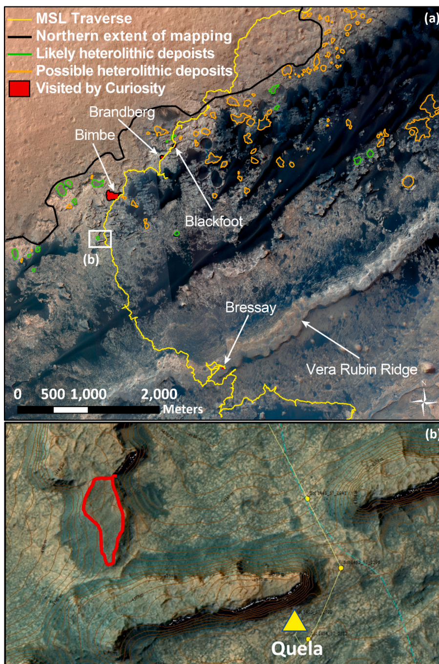
Fig. 24. Location of heterolithic units of un lithified gravel deposits. a) HiRISE orthoimagery overlain by likely (green), possible (orange) and visited (red) heterolithic units (e.g., Wiens et al., 2020 ). b) The Quela area where a heterolithic unit (red outline) is deposited on top of both the Murray and Stimson formations and Martin et al. (2021) report an exposure of 1 billion years (located at the triangle). HiRISE image credit: NASA/JPL/University of Arizona. (For interpretation of the references to colour in this figure legend, the reader is referred to the web version of this article.)
