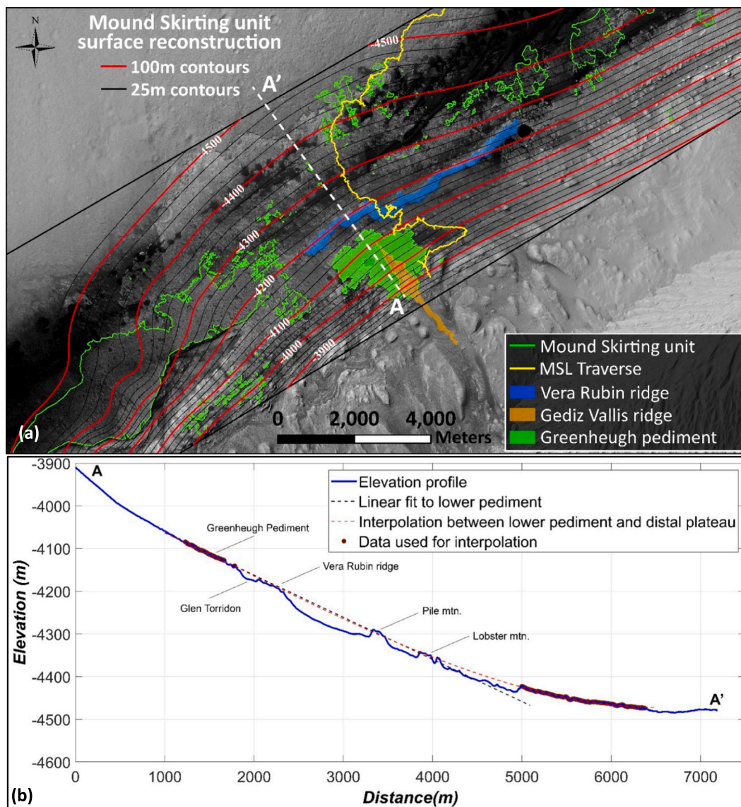
Fig. 22. Mound Skirting unit surface reconstruction prior to erosional dissection. a) HiRISE orthoimagery overlain with 25- and 100-m contours of the reconstructed Mound Skirting unit. Modern exposures of the Mound Skirting unit (equivalent to the SPg group in this area) are shown outlined in green. The Greenheugh pediment, Vera Rubin ridge, and the Gediz Vallis ridge are shaded in green, blue, and orange respectively. Projection assumes all the Mound Skirting Unit outcrops and Stimson mantled Greenheugh pediment were part of a footslope aeolian dune field (Stimson fm.). b) Topographic profile A-A' (see (a)) with labeled locations and two reconstructions (linear and 2nd order polynomial fits) of the Greenheugh pediment (Reproduced from Bryk et al., 2019b). Red dots indicate topographic data used for the polynomial fit. HiRISE image credit: NASA/JPL/University of Arizona. (For interpretation of the references to colour in this figure legend, the reader is referred to the web version of this article.)
