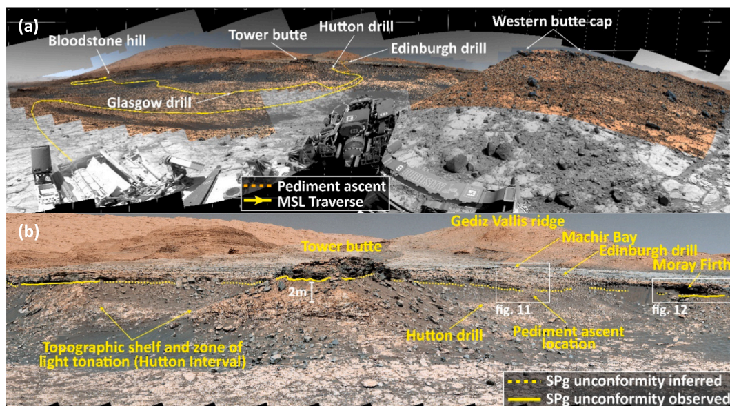
Fig. 10. Mastcam imagery overlain on Navcam imagery taken from the northeast ‘shoulder’ of Western butte towards the Greenheugh pediment and centered on Tower butte a) Context (180°) view of pediment ascent area as viewed from the shoulder of Western butte. The pediment ascent location, Hutton, Edinburgh and Glasgow drill sites, and Bloodstone hill can also be seen along the MSL traverse (yellow/orange) (mixture of M100 and Navcam imagery). b) Closer view of the ascent area at Tower butte. Image credit: NASA/JPL-Caltech/MSSS. See Table S1 in Supporting information S3 for image sequence identifiers. (For interpretation of the references to colour in this figure legend, the reader is referred to the web version of this article.)
