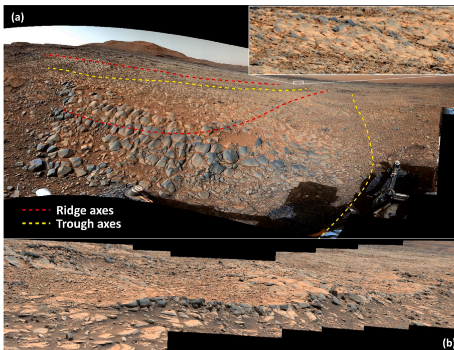
Fig. 19. Pediment surface at the Blackcraig ascent area a) Ridges (red) and troughs (yellow) and prominent ventifaction pattern (“gatorback”) characteristic of intact washboard Stimson. Inset shows gatorback pattern present near the base of the Gediz Vallis Ridge b) A cross-sectional view of the washboard pattern suggesting a relationship between the topography Stimson internal stratigraphy. Mastcam image credit: NASA/JPL-Caltech/MSSS. See Table S1 in Supporting information S3 for image sequence identifiers. (For interpretation of the references to colour in this figure legend, the reader is referred to the web version of this article.)
