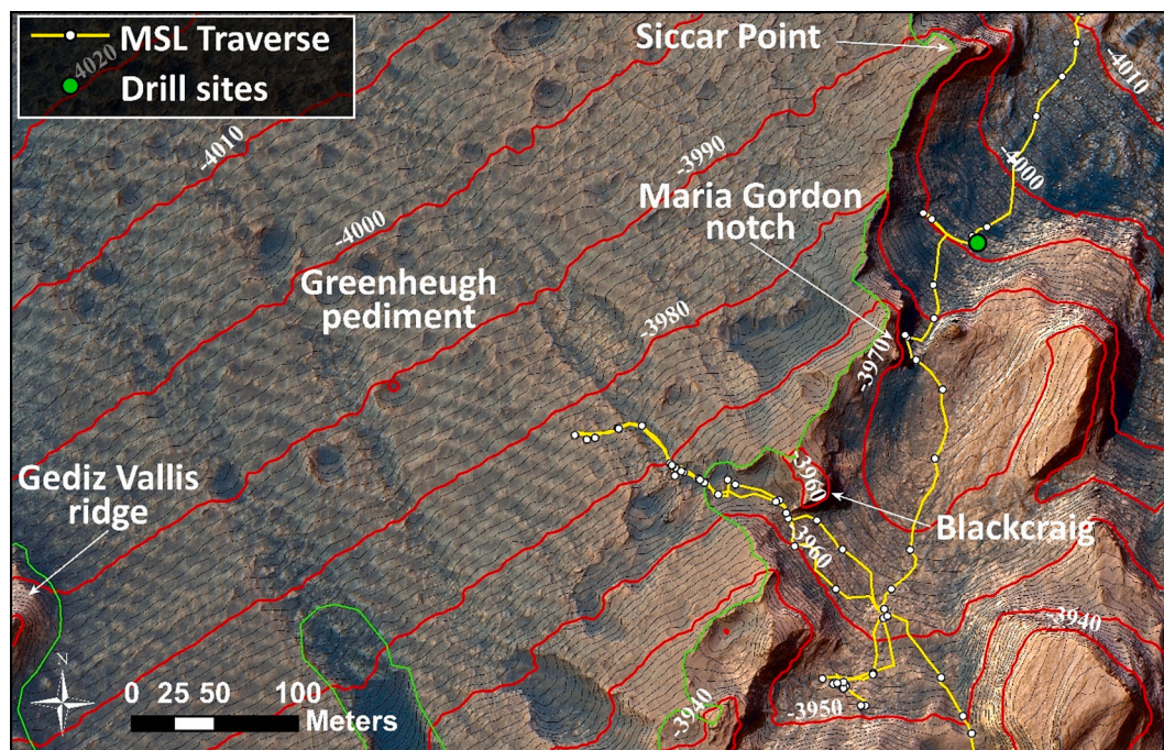
Fig. 17. Map showing the Southern pediment ascent at Blackcraig. The green line delineates pediment edge and the yellow line indicates the rover path. HIRISE image credit: NASA/JPL/University of Arizona. (For interpretation of the references to colour in this figure legend, the reader is referred to the web version of this article.)
