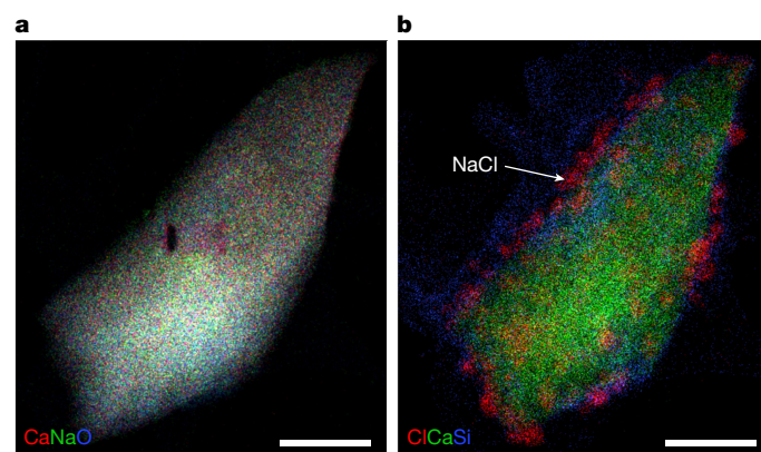
Fig. 2 | Hydrated Na, Ca carbonate. a , Na, Ca carbonate grain, studied about 1 month following removal from nitrogen storage in the curatorial facility, exhibits SAED d -spacing consistent with the hydrated phases gaylussite or pirssonite. The mineral is sensitive to beam damage (dark spot within grain), consistent with a hydrated phase (multi-element \text{K}\alpha X-ray map; sample no. OREX-800045-102). b , NaCl particles grown on the same grain after 5 months (multi-element \text{K}\alpha X-ray map). Scale bars, 200 nm.
