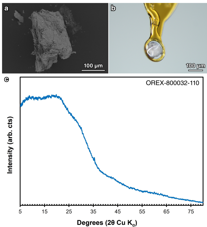
Extended Data Fig. 5 | X-ray diffraction demonstrates that Mg,Na phosphate is poorly crystalline or amorphous. (a) SEMBSE image of Mg,Na phosphate OREX-800032-110 mounted on a carbon adhesive disc. (b) Optical image of the particle fixed to a Kapton loop using a small amount of glue. (c) Micro-XRD pattern acquired from the same particle showing the lack of coherent diffraction. A small diffraction peak at \sim 35^\circ ( 2\theta ) may be related to matrix material adhering to the surface of the particle.
