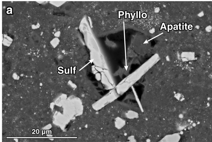
Extended Data Fig. 1 | Early-forming phases during water-rock interactions on Benuu. (a) Subhedral void with co-existing sulfide laths/blades, apatite, and fibrous phyllosilicates (BSE image; OREX-501062-100). (b) Calcites of near-end
