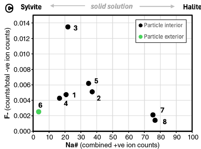
Extended Data Fig. 7 | Halite and sylvite grains in Benu sample OREX-501070-0. (a) SE image of halite- and sylvite-bearing particle subjected to FIB milling. (b) BSE image of the particle in (a) after FIB-milling the top 10 μm, revealing Ca-Mg-Fe-Ti-Al-bearing clinopyroxene, plagioclase, halite, and
