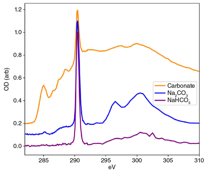
Extended Data Fig.3 | STEM spectrum (orange) of a carbonate-rich region of phyllosilicate matrix. STEM EDS shows that the outlined region in Fig. 1c contains abundant carbon, 0.5 at.% Na, and detectable K. The between 295 and 305 eV shows features not typical of pure organics but consistent with carbonates. The Na 2 CO 3 (blue) and NaHCO 3 (purple) standards were prepared by allowing ~1 μL of dissolved powder in deionized water to evaporate on a TEM grid. The centroid of the carbonate peak is at 290.50 for Na 2 CO 3 , 290.47 for NaHCO 3 , and 290.46 for Bennu showing excellent experimental agreement.
