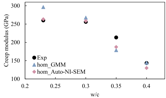
Figure 19. Creep modulus of the four cement pastes, experimental and homogenized, as a function of the water-to-cement ratio.
