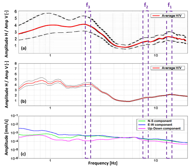
Figure 2. Visualization of (a) Global spectrum amplitude ratio H/V across all sensors, (b) Individual spectrum amplitude ratio H/V from a single sensor, and (c) Spectrum amplitude by direction from the single sensor
