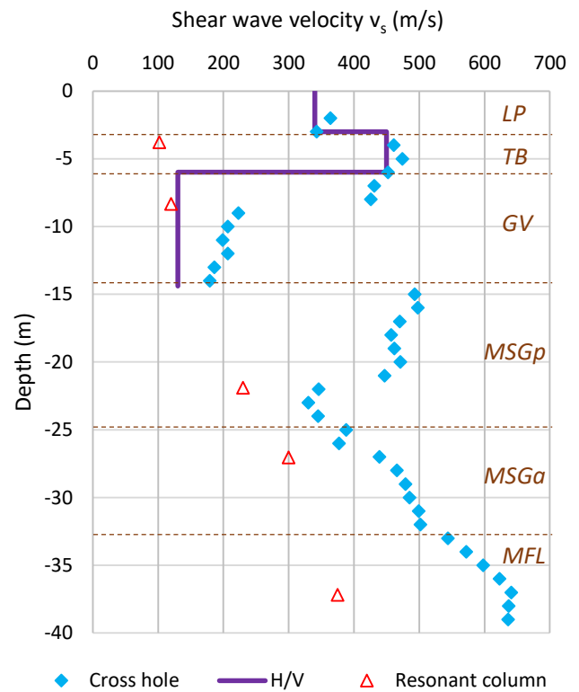
Figure 4. Shear wave velocities measurements
