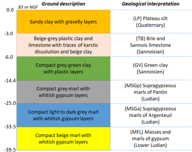
Figure 1. Geological profile (scale not observed). 83 NGF correspond to the surface of the work site.
