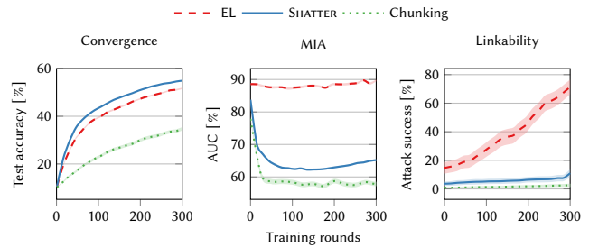
Figure 9: Ablation study: convergence and resistance against MIA and LA with different components of SHATTER enabled.
