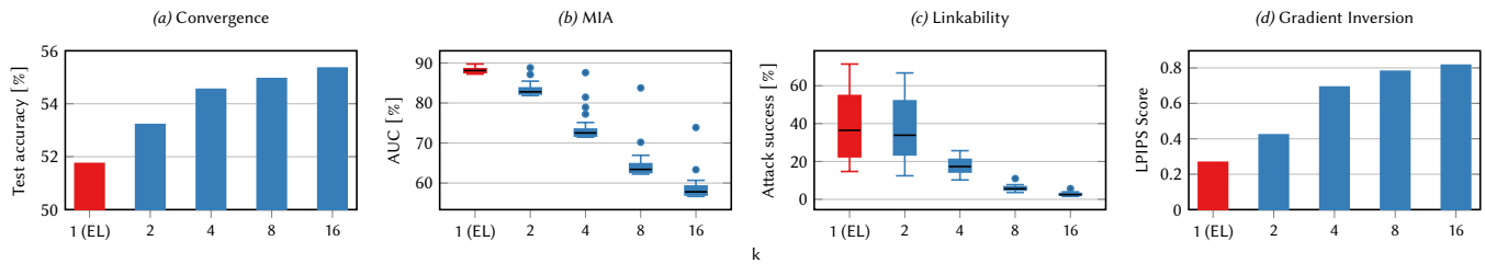
Figure 7: The test accuracy (a, ↑ is better), MIA AUC (b, ↓ is better), attack success rate for LA (c, ↓ is better) on CIFAR-10, and GIA LPIPS score (d, ↑ is better) on ImageNet for increasing values of k (with k = 1 corresponding to an EL setting).
