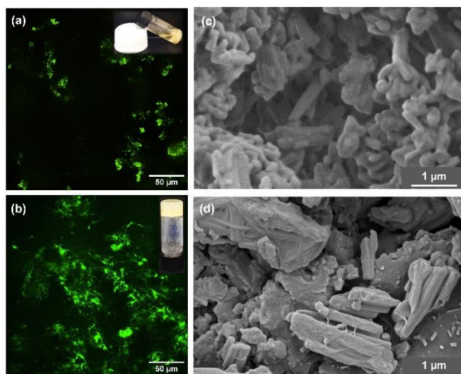
Fig. 1 CLSM microscopy images of (a) stained GlcBMe + Ar + H 2 O – mix before sonication then (b) stained GlcBMe-Ar oleogel; and SEM images of (c) as-prepared GlcBMe then (d) GlcBMe oleogelator obtained from oleogel washed out with acetone
