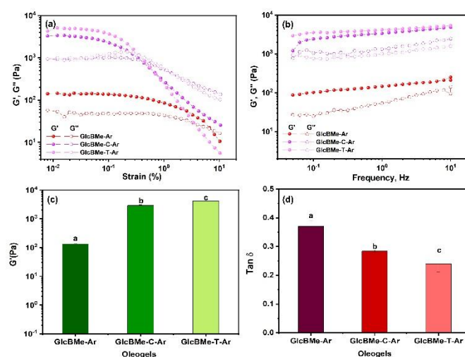
Fig. 4 Rheological behavior of oleogels (a) Strain sweeps (b) Frequency sweep (c) G' vs. oleogels (d) \tan \delta vs. oleogels for samples GlcBMe-Ar, GlcBMe-C-Ar, GlcBMe-T-Ar. Different letters assigned to each bar represent statistical differences between the values across all samples ( p < 0.05 )
