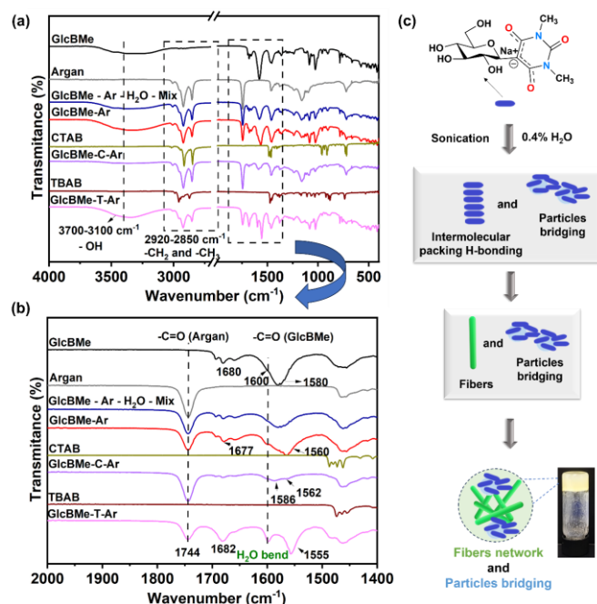
Fig. 2 a) IR spectra (4000-450 \text{cm}^{-1} ) and (b) (2000-1400 \text{cm}^{-1} ) of GlcBMe, argan oil, GlcBMe-Ar-H 2 O-mix, GlcBMe-Ar, CTAB, GlcBMe-C-Ar, TBAB and GlcBMe-T-Ar (c) Illustration of self-assembly mechanism
