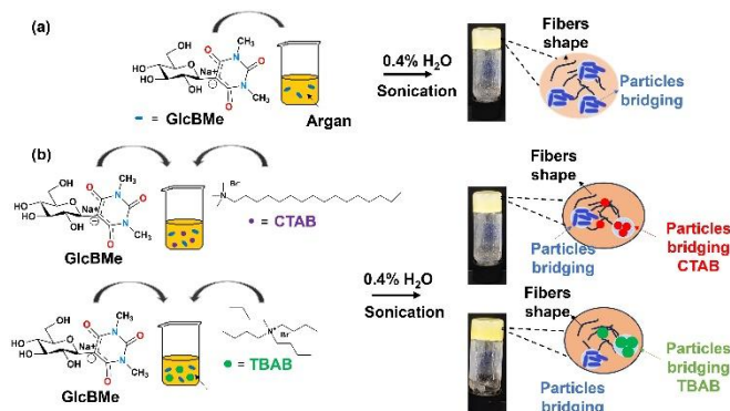
Scheme 2 Mechanism of formation of (a) GlcBMe-based oleogel in argan oil and (b) GlcBMe-based oleogels with cationic surfactants and different oils
