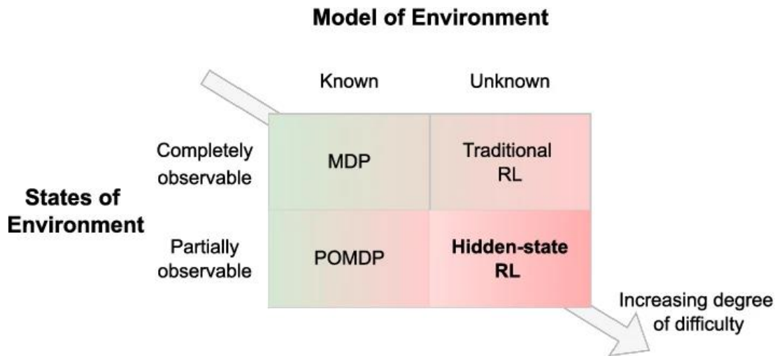
Fig. 2. Increasing Degree of Difficulty for RL agent in Predictive Maintenance (Siraskar et al. 2023)
