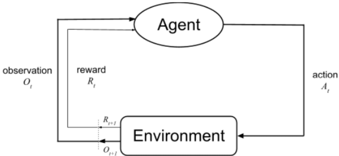
Fig. 1. RL cycle (Agent-Environment Interaction), showing observation (state), actions, rewards, policy updates, and the feedback loop [71]
