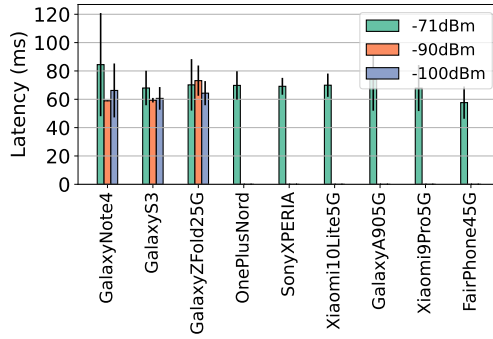
Figure 11: Indoor network authentication latency per phone model w.r.t. the signal quality.
