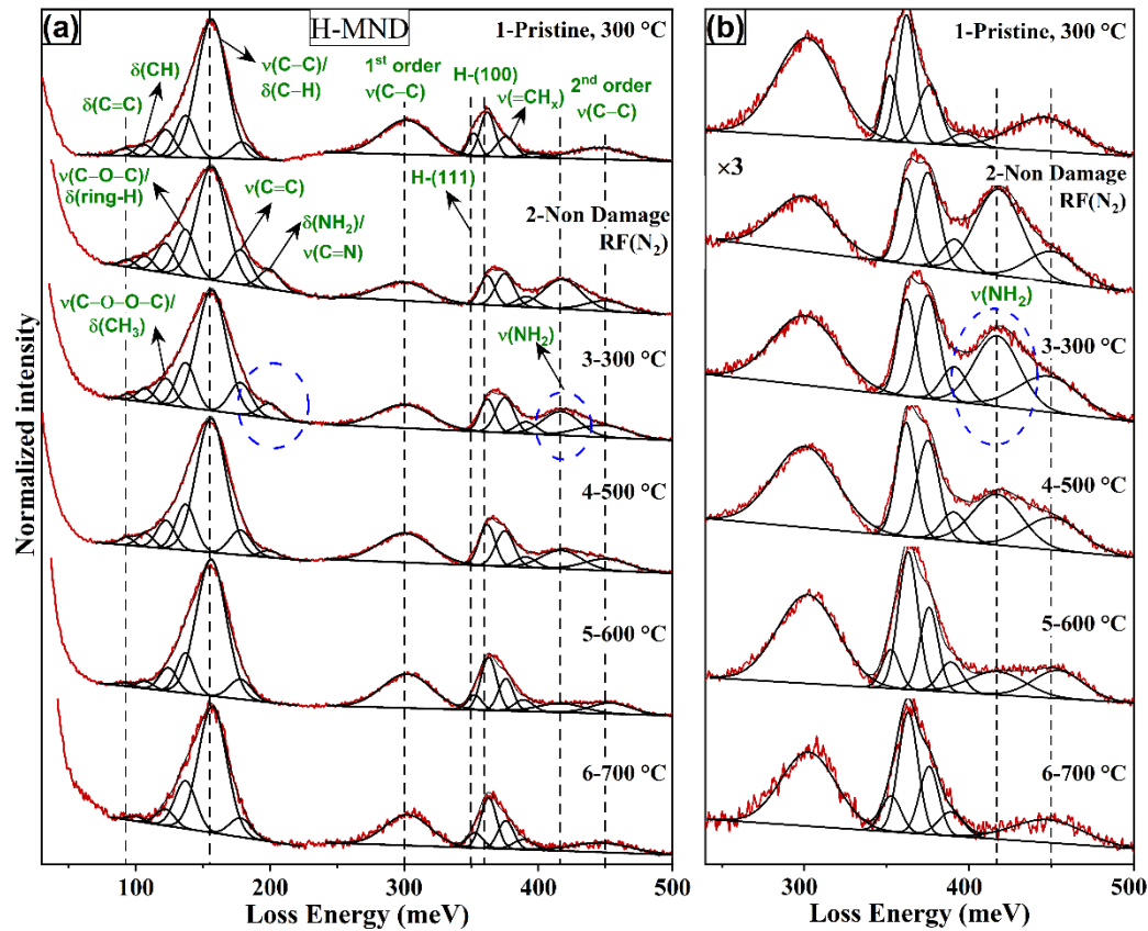
Figure 4. (a) HREEL spectra of H-MND surface exposed to non-damage RF(N 2 ) plasma and subsequently annealed at different temperatures. (b) ×3 magnified (in the y-axis) spectra of (a) in the range 230–500 meV.
