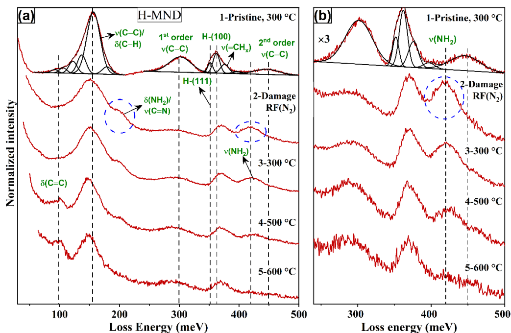
Figure 5. (a) HREEL spectra of H-MND surface exposed to damage RF(N 2 ) plasma and subsequently annealed at different temperatures. (b) ×3 magnified (in the y-axis) spectra of (a) in the range 230–500 meV.
