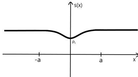
Figure 1: Function s(x)
