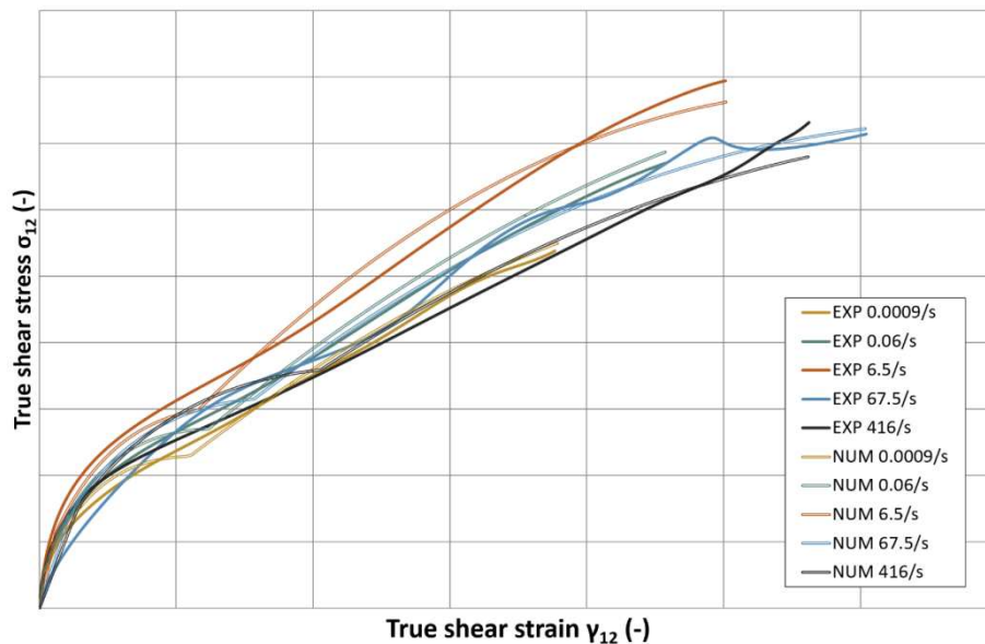
Figure 5. Comparison dynamic experiments/numerical simulations for the 45° fabric at 23°C and RH=50%.
