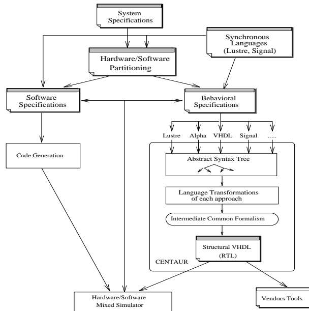
Figure 1: Overall structure of ASAR
