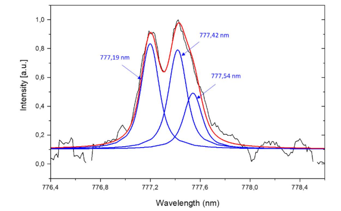
Oxygen lines deconvolution at r = 30 μm, over Δz = 300μm from the pin. Time integration is 3 ns from 5 ns after the start of the discharge.
