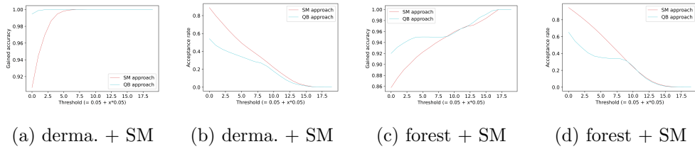
Fig. 6 Test accuracy and acceptance rate as the functions of the threshold: 20 \times 5 cross-validation with (train, test) = (20%, 80%) on noisy data sets
