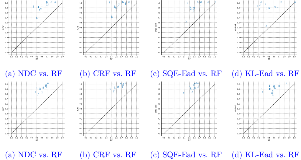
Fig. 7 Correctness of different imprecise classifiers in the case of abstention versus accuracy of the random forest on training sets without noise (first row) and with 25% noise (second row).
