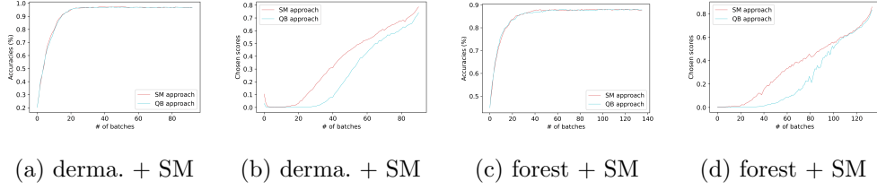
Fig. 3 Test accuracy and chosen score as the functions of the number of queries: 10 \times 5 cross-validation with (train, pool, test) = (3%, 77%, 20%) on noisy data sets
