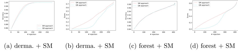
Fig. 5 Test accuracy and chosen score as the functions of the number of rejections: 20 \times 5 cross-validation with (train, test) = (20%, 80%) on noisy data sets
