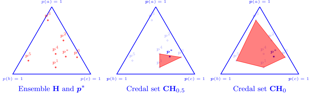
Fig. 1 Illustration of \mathbf{CH}_\alpha(\mathbf{x}) for \mathcal{Y} = \{a, b, c\} .
