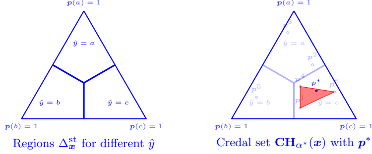
Fig. 2 Illustration of \Delta_{\mathbf{x}}^{\text{st}} for 0/1 loss (5) and of \mathbf{CH}_{\alpha^*}(\mathbf{x}) .
