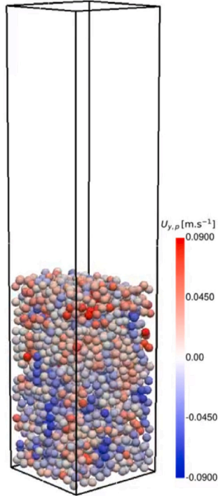
Fig. 9. Snapshot of a simulation at the highest solid fraction ( \alpha = 0.36 , U_f = 0.073 \text{ m s}^{-1} ).
