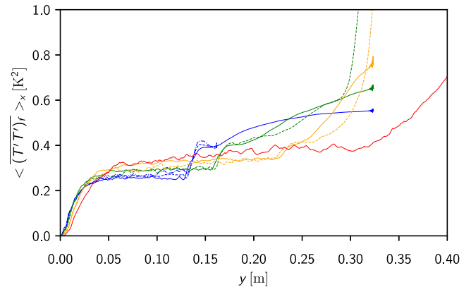
Fig. 14. Profile of the double temperature correlation along the bed height for different fluidization velocities U_f and mesh resolutions \frac{D_x}{\Delta x} . —: U_f = 0.073 \text{ m s}^{-1} , —: U_f = 0.09 \text{ m s}^{-1} , —: U_f = 0.12 \text{ m s}^{-1} , —: U_f = 0.15 \text{ m s}^{-1} . —: \frac{D_x}{\Delta x} = 12 , - -: \frac{D_x}{\Delta x} = 24 , - ·: \frac{D_x}{\Delta x} = 36 . For all mesh resolution, curves are superimposed along the bed height.
