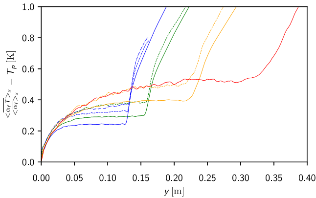
Fig. 13. Mean temperature profile along the bed height for different fluidization velocities U_f and mesh resolutions \frac{D_x}{\Delta x} . —: U_f = 0.073 \text{ m s}^{-1} , —: U_f = 0.09 \text{ m s}^{-1} , —: U_f = 0.12 \text{ m s}^{-1} , —: U_f = 0.15 \text{ m s}^{-1} . —: \frac{D_x}{\Delta x} = 12 , - -: \frac{D_x}{\Delta x} = 24 , - ·: \frac{D_x}{\Delta x} = 36 .
