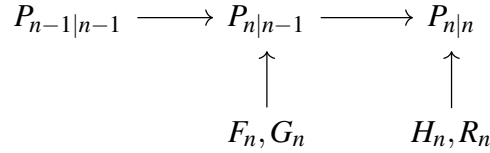
Figure 7: Dependencies of KF's variables in Riccati's equations
