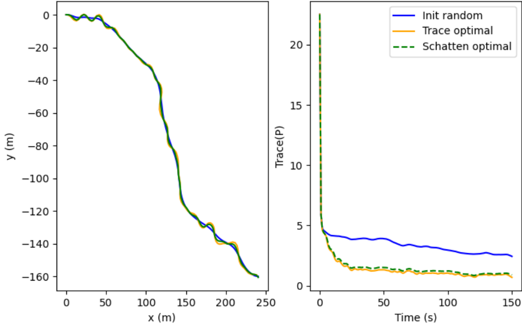
Figure 3: On the left, an example of an initial random guess in blue. The other two trajectories are solutions to the perception-aware problem where the loss is the trace (in orange) and the Schatten norm (in green). The right plot shows the expected trace of the covariance evolution for each trajectory.
