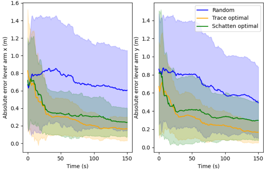
Figure 4: Absolute estimation error of the lever arm during the trajectory. On the left the error for the lever arm in x and on the right in y. One- \sigma envelope illustrates the dispersion of errors over trials.
