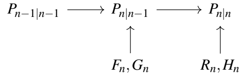
Figure 1: Dependencies of EKF's variables in Riccati equations (3) and (8). Each variable (node) is a function of its predecessors.
