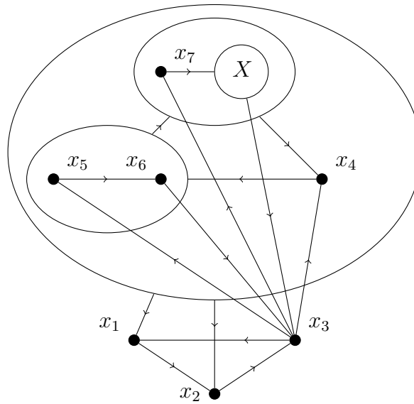
Figure 6: Tournament W with X an all-kings (n - 7) -tournament
