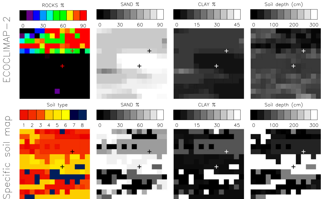
FIG. 3. Soil maps used for the ALMIP2 simulations over the Mali site. (top) Rocks fraction, soil texture, and depth from the ECOCLIMAP2 dataset. (bottom) Soil types, soil texture, and depth from the specific soil classification developed for this study. Plus signs indicate the position of sites 17 and 40.
