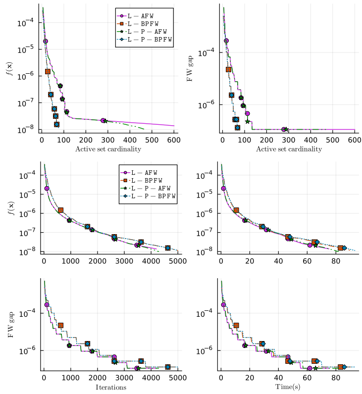
Figure 3: K -sparse logistic regression, K = 10 and \tau = 1.0 .
