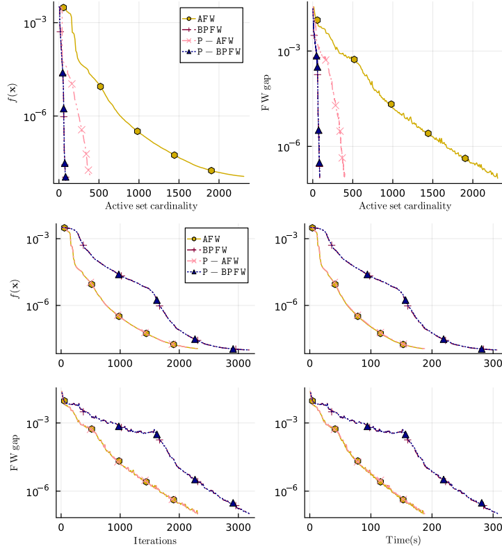
Figure 2: Logistic regression, \tau = 60 .
