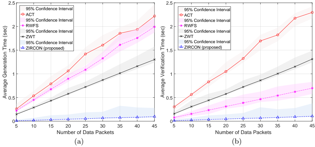
Fig. 9: Computational time. (a) Watermark generation and embedding time. (b) Watermark verification time.
