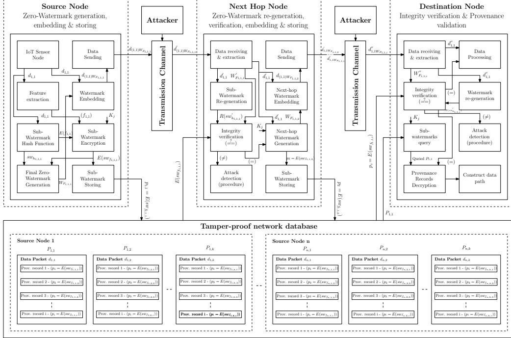
Fig. 4: Zero-watermark generation, storing and verification block diagram in multi-hop scenario.
