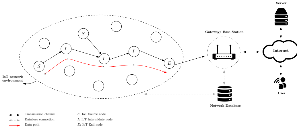
Fig. 2: Multi hop network model.
