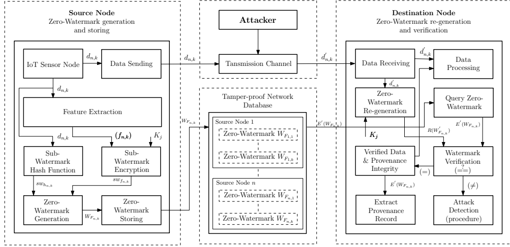
Fig. 3: Zero-watermark generation, storing and verification block diagram in single hop scenario.
