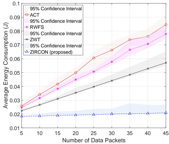
Fig. 11: Energy consumption cost per single source node.
