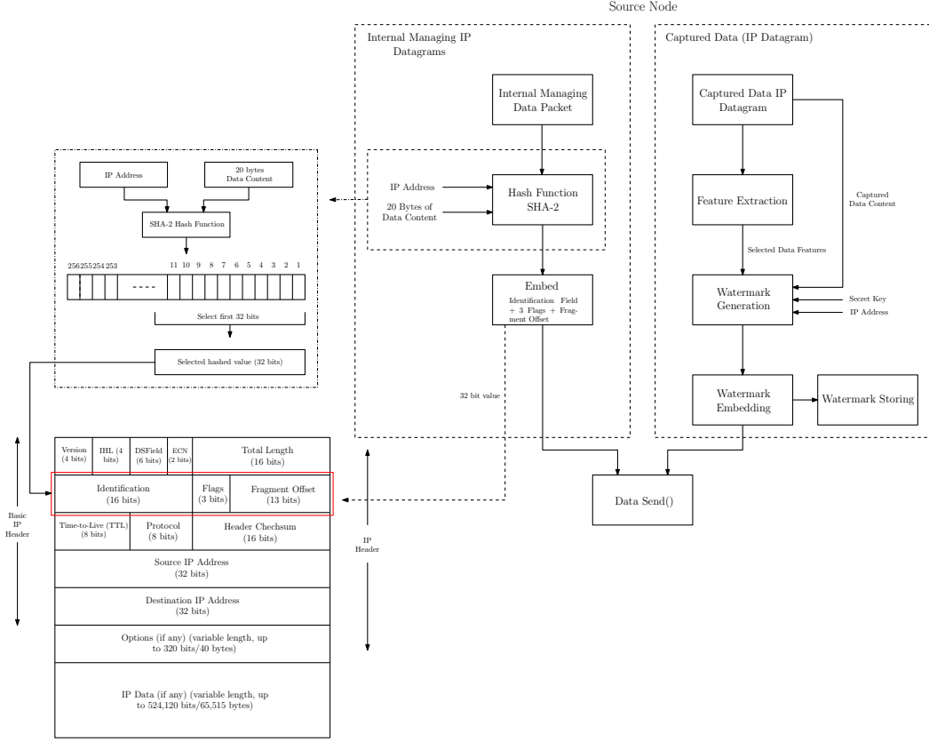
Fig. 5: Embedding hash value in Internal Managing Protocol.
