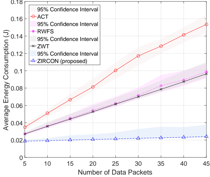
Fig. 12: Energy consumption cost per single intermediate node.
