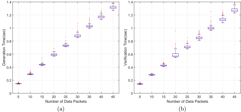
Fig. 7: Computational time. (a) Watermark generation and embedding time using DES. (b) Watermark verification time using DES.
