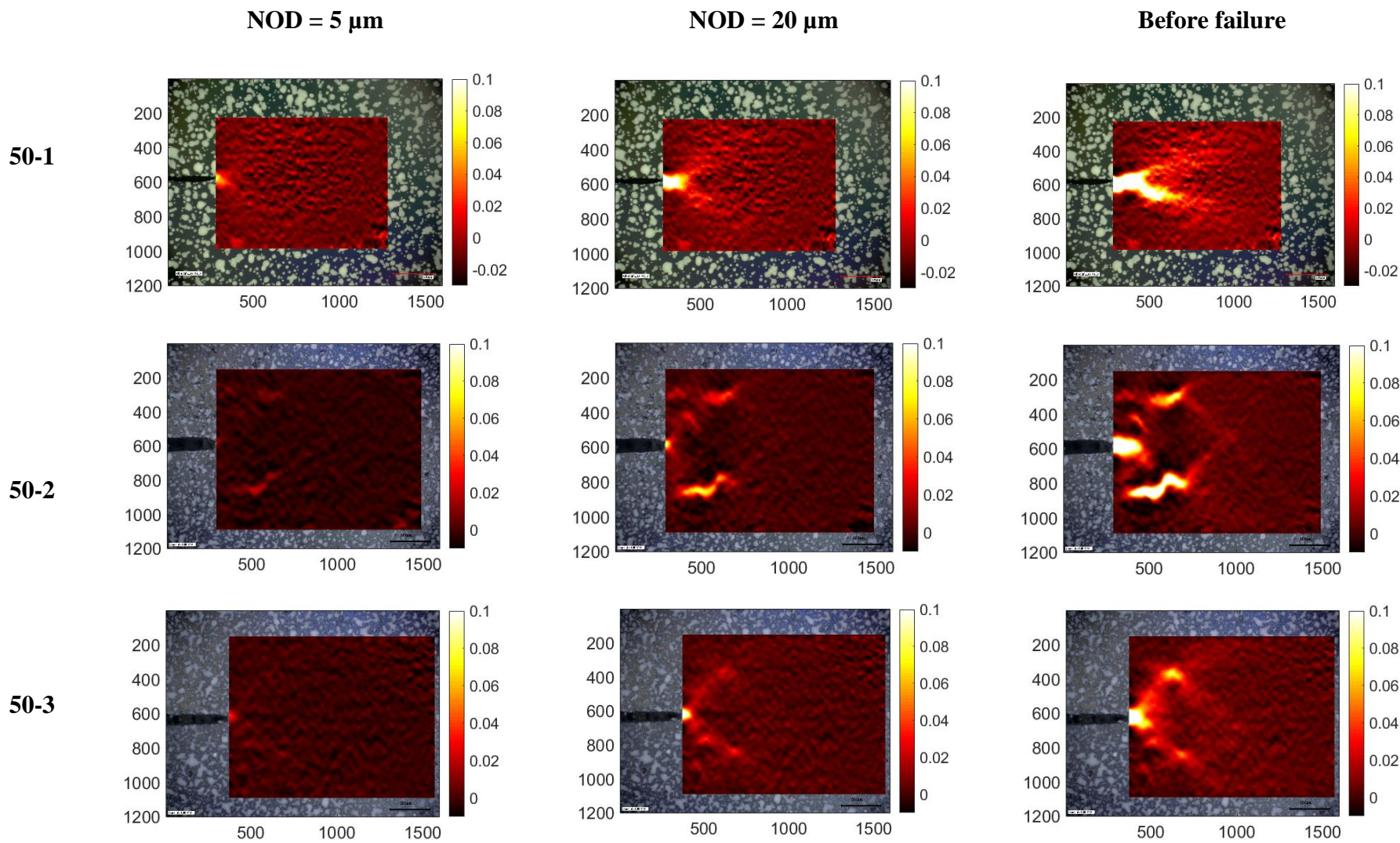
Figure 8: Strain maps for specimens with 50 μm thickness at different NOD levels.
