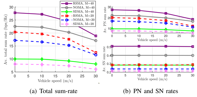
Fig. 2: Total, PN, and SN sum-rates for varying vehicle speeds
