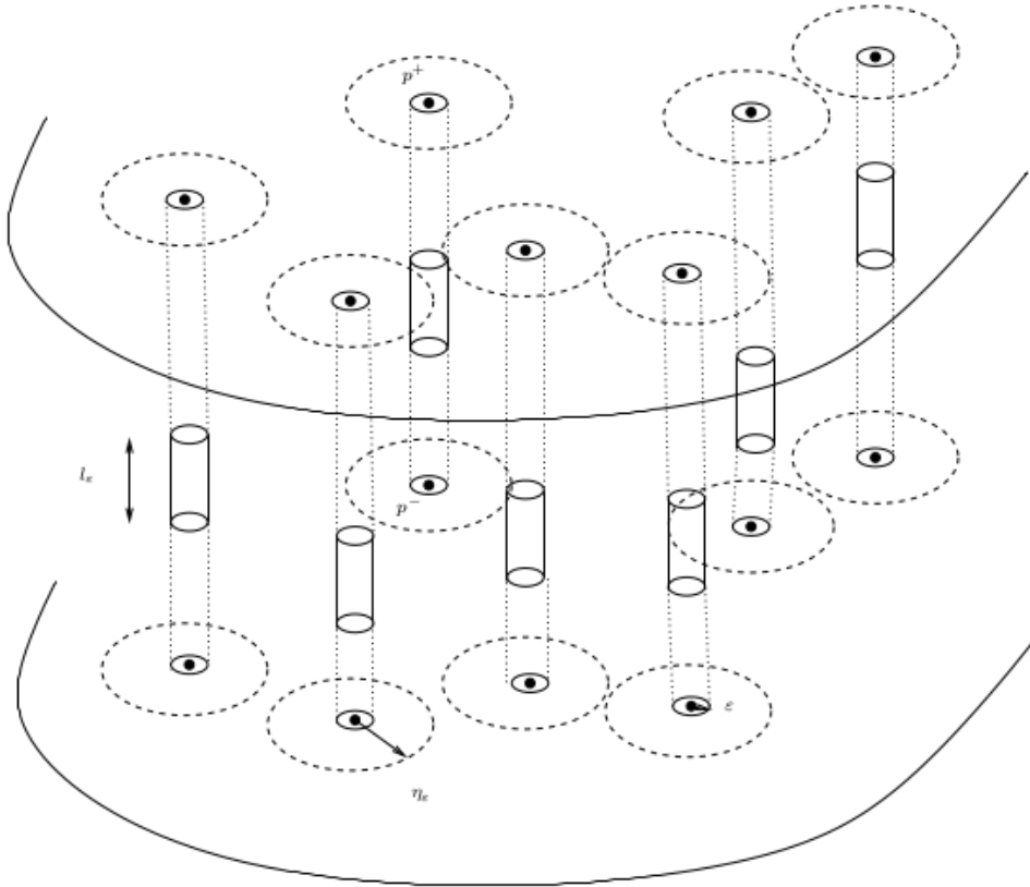
FIGURE 1. The manifold M_\varepsilon obtained from X (here the top and lower flat region) by removing many small balls B_\varepsilon(p) of radius \varepsilon by attaching handles C_\varepsilon(p) . The small dotted lines mean identification.
