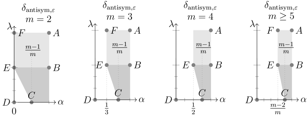
FIGURE 10. The range of the parameters \alpha and \lambda where \delta_{\text{antisym},\varepsilon} (appearing in Lemma 6.2) converges. The light grey (infinite) rectangle ABEF is of order O(\varepsilon^{(m\alpha-(m-2))/2}) ; the dark grey polygon C(1,0)BE is of order O(\varepsilon^{(\lambda+m\alpha-(m-1))/2}) .
