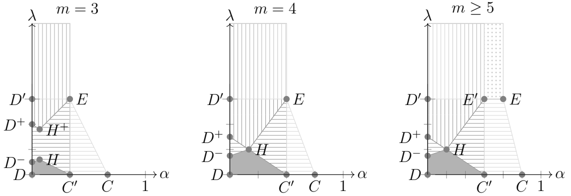
FIGURE 4. Comparison of the two fading results: horizontal light lines: only Corollary 3.5 applies; vertical light lines: only Corollary 3.2 applies; horizontal dark lines: Corollary 3.5 has better estimates than Corollary 3.2; vertical dark lines: Corollary 3.2 has better estimates than Corollary 3.5; grey area: both results have the same order on the convergence speed. Dotted area (only for m \geq 5 ): none of our results apply.
