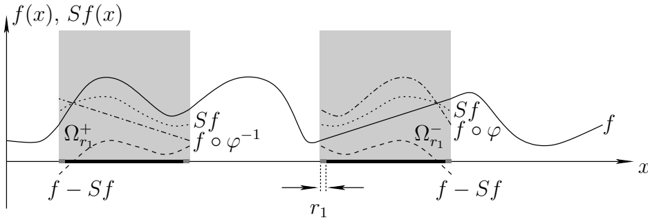
FIGURE 11. The symmetrisation operator S changing f on \Omega_{r_1} = \Omega_{r_1}^+ \cup \Omega_{r_1}^- (fat grey and black line, in grey: \Omega = \Omega^+ \cup \Omega^- ); shaded in grey in the diagram. Here, the diagram is plotted for x \in X along the dotted line of Figure 5. full line : the original function f . Dotted : The symmetrised function Sf (only changed on \Omega_{r_1} ). Dashed : The anti-symmetric part f - Sf of f . Dotted-dashed : The function f copied from the other isometric set.
