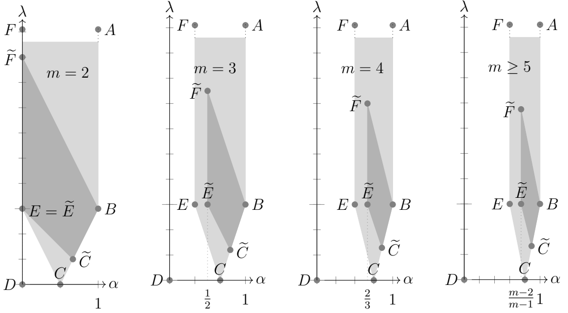
FIGURE 7. The range inside B\tilde{F}\tilde{E}\tilde{C} is the range covered by our adhering case Corollary 3.14 (dark grey). The parameter range covered by [Kh13, Thm. 2.6] is given by the (unbounded) polygon ABCEF (lighter grey), see Remark 3.20.
