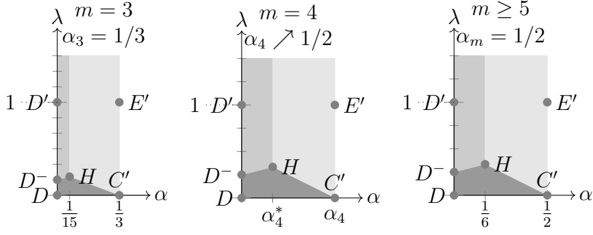
FIGURE 2. The range of the parameters \alpha ( \eta_\varepsilon = \varepsilon^\alpha r_0 , the larger the denser the handles are) and \lambda ( \ell_\varepsilon = \varepsilon^\lambda , the larger the shorter the handles are) in which Corollary 3.2 is valid ( m \geq 3 ). For the letters describing points in the (\alpha, \lambda) -plane, see (3.2)). The estimate on the convergence speed is of order O(\varepsilon^{(\alpha_m - \alpha)/(2(1 - \alpha_m)}) in the (infinite) rectangle C'G(\alpha_m^*, \infty)(\alpha_m, \infty) (lightest grey), of order O(\varepsilon^{(\alpha_m + \alpha)/2}) in the (infinite) rectangle D^-(0, \infty)(\alpha_m^*, \infty)G (middle grey) resp. of order O(\varepsilon^\lambda) in the triangle C'DD^-G (dark grey).
