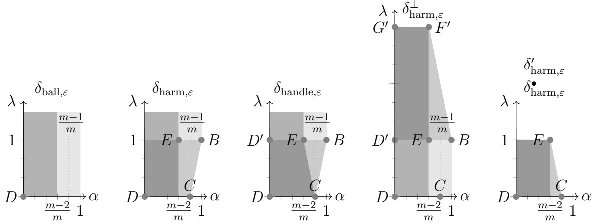
FIGURE 9. The range of the parameters \alpha and \lambda for the various constants. Darkest grey: Second left : O(\varepsilon^{(\lambda+1)/2}) , middle : O(\varepsilon^\lambda) , second right : O(\varepsilon^{(3-\lambda)/2}) , right : O(\varepsilon^{(1-\lambda)/2}) . Second darkest grey: Left, second left, middle and second right : O(\varepsilon) . Second lightest grey: Second left and middle : O(\varepsilon^{(\lambda+(m-1)-\alpha m)/2}) , second right : O(\varepsilon^{1-\lambda+(1-\alpha)m/2}) , right : O(\varepsilon^{(-\lambda+(m-1)-\alpha m)/2}) . Lightest grey: Left, second left, middle and second right : O(\varepsilon^{m(1-\alpha)/2}) .
