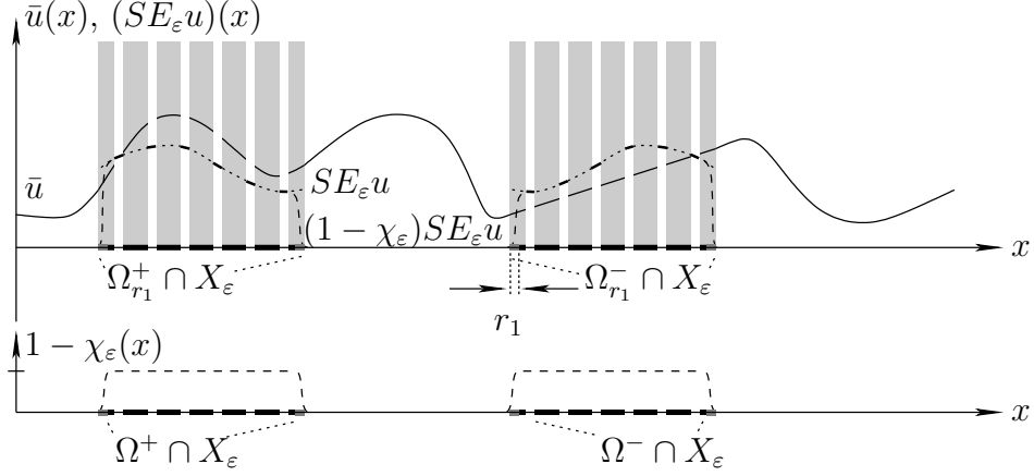
FIGURE 12. The identification operators J'_\varepsilon and J_\varepsilon^1 and its ingredients: \bar{u} (full line) is the extension by 0 onto B_\varepsilon ; SE_\varepsilon u (dotted and thick line) is the symmetrisation of the harmonic extension of u and (1 - \chi_\varepsilon)SE_\varepsilon u (dashed) is the smoothed function symmetric on \Omega using the cut-off function 1 - \chi_\varepsilon with support in \Omega_{\bar{\varepsilon}} .
