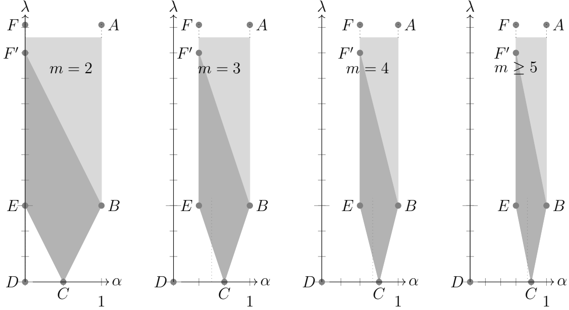
FIGURE 8. The range inside BFEC is the range covered by our simplified adhering case Corollary 3.18 (dark grey). Here, “simplified” means that X consists only of two isometric manifolds \Omega^- and \Omega^+ . The parameter range covered by [Kh13, Thm. 2.6] is again inside the polygon ABCEF (lighter grey).
