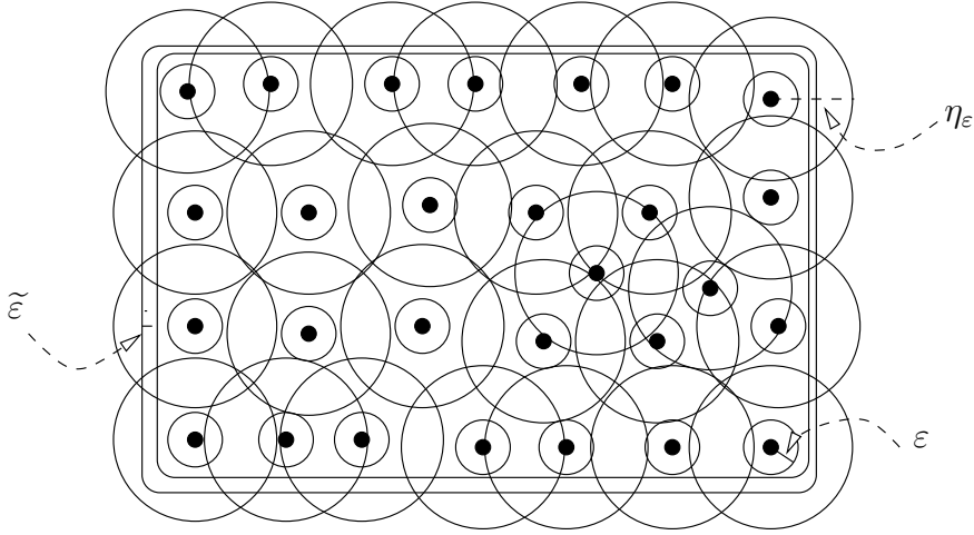
FIGURE 6. The covering of \Omega_\varepsilon^\pm with \eta_\varepsilon -cover number N = 3 .
