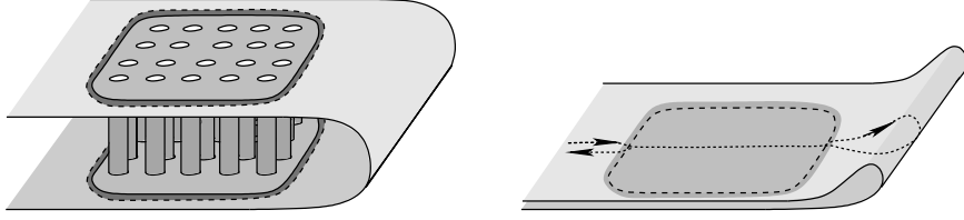
FIGURE 5. Left: The manifold M_\varepsilon with handles of radius \varepsilon and length \ell_\varepsilon ; medium grey: \Omega^+ (top) and \Omega^- (bottom), together with its \tilde{\varepsilon} -neighbourhood \Omega_{\tilde{\varepsilon}}^+ and \Omega_{\tilde{\varepsilon}}^- in medium and dark grey, respectively.
