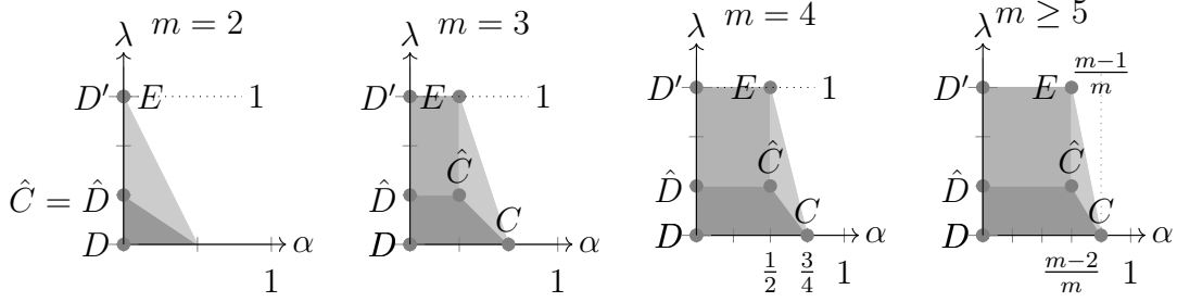
FIGURE 3. The range of the parameters \alpha ( \eta_\varepsilon = \varepsilon^\alpha r_0 in which Corollary 3.5 is valid. The estimate on the convergence speed is of order O(\varepsilon^{(1 - \lambda)/2}) in the polygon C'DD^-G (horizontal lines); of order O(\varepsilon^{(-\lambda + (m-1) - m\alpha)/2}) in the polygon (diagonal lines) resp. of order O(\varepsilon^\lambda) (dark grey).
