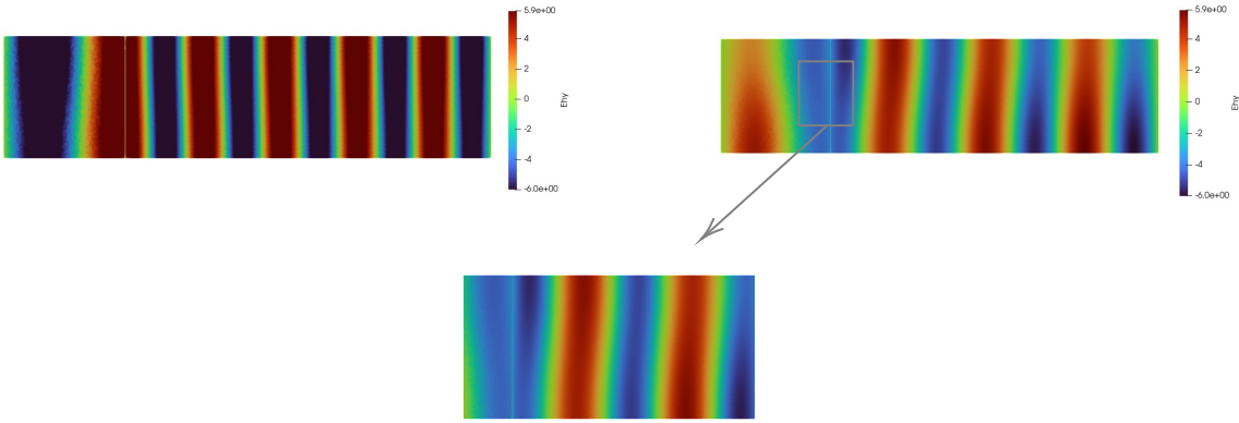
Figure 10 The y -component of the approximate solution \mathbf{E}_h obtained with the volume optimal control method ([Left] \kappa_\varepsilon = -2 ; [Right] \kappa_\varepsilon = -1 ).
