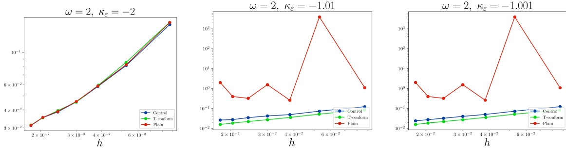
Figure 5 Comparison of the three relative errors (control, T -conform, plain) with respect to the mesh size h .
