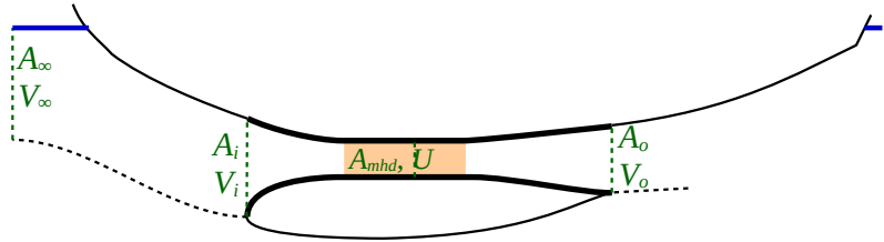
Figure 4. Propulsion channel of a MHD boat
