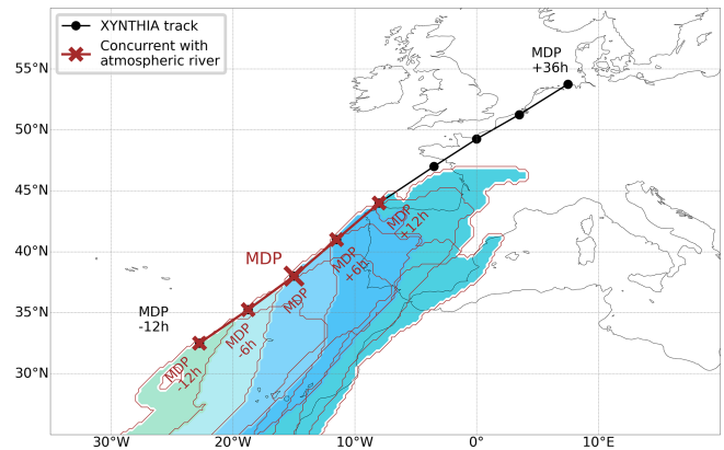
Figure 3. Example of the detection and tracking of an EC (Xynthia, 26 February 2010 at 18:00 UTC to 1 March 2010 at 00:00 UTC) concurrent to an AR in ERA5. Red crosses mark the location of the cyclone at times when it concurred with an AR. Black dots indicate no concurrence. Shaded areas depict the regions identified as ARs at each concurrence time step during the cyclone trajectory.
