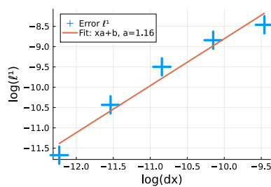
(A) Numerical convergence for the model without the viscous term.
