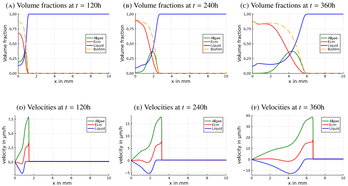
FIGURE 4. Mixture components volume fractions (first row) and velocities (second row) for different times. In this simulation, the viscosity is included and the elastic tensors for the biological phases are multiplied 9 \cdot 10^7 so the biofilm front velocity matches experimental measurements. The simulation is made using 2048 mesh cells for the space grid.
