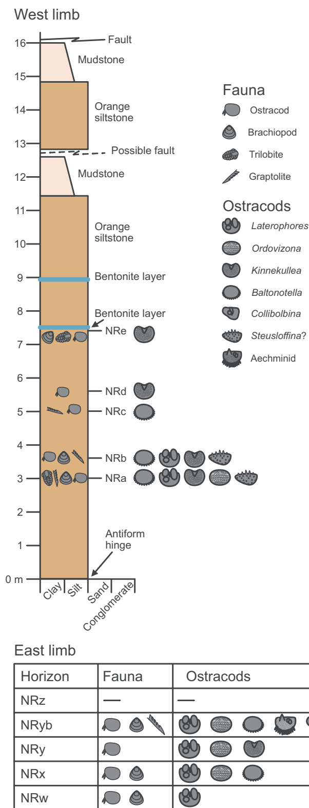
FIGURE 2 | Stratigraphic log of the west limb of the anticline accessible in the Na Ri district section of the Phu Ngu Formation (top) and table showing the distribution of fauna and ostracod taxa recovered from the horizons of the east limb (bottom).
