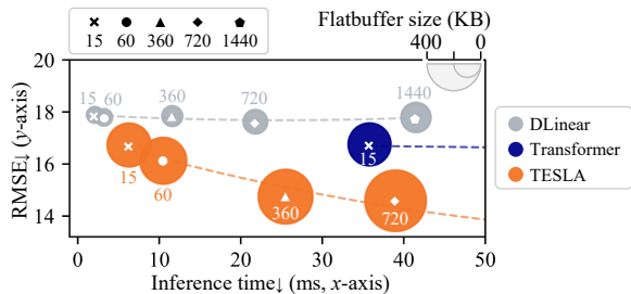
Figure 6: Evaluation of the Arduino Nano 33 BLE Sense microcontroller. The scatter map illustrates RMSE, inference time, and Flatbuffer size (diameter of the circles) with varying windows (15, 60, 360, 720, 1440) for average \text{PM}_{10} performance across three regions. Missing window sizes indicate non-applicability. The dotted line represents the trend.
