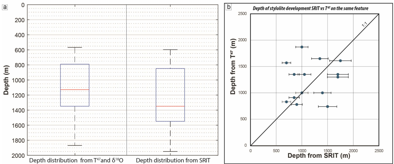
Figure 7. (a) Box plots of the range of depths for pressure solution from (left-side) isotope thermometry (measured T_{47} and calculated from \delta^{18}\text{O} values, see text for details, assuming a geothermal gradient of 23\text{ }^\circ\text{C}/\text{km} and a surface temperature of 10\text{ }^\circ\text{C} ) applied on syn-solution development and filling of jogs at stylolite tips ( n = 27 , left-side) and from SRIT on BPS ( n = 31 , right-side). Represented from top to bottom are the minimum value, the first quartile, the median (red), the third quartile and the maximum value of the range. The dotted grid represents 50\text{ m} intervals. (b) Plot of depth of stylolite development for coupled stylolite/jogs. Each blue dot represents a couple ( n = 14 ). Error bars are calculated to be 12\% of the depth value obtained from SRIT.
