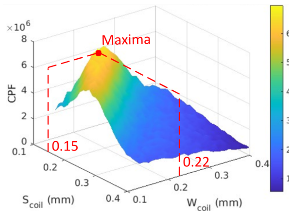
Figure 12. Three-turn coil’s CPF as a function of W_{coil} and S_{coil} .
