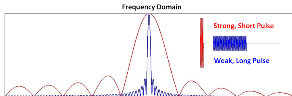
Figure 6. Pulse bandwidth.
