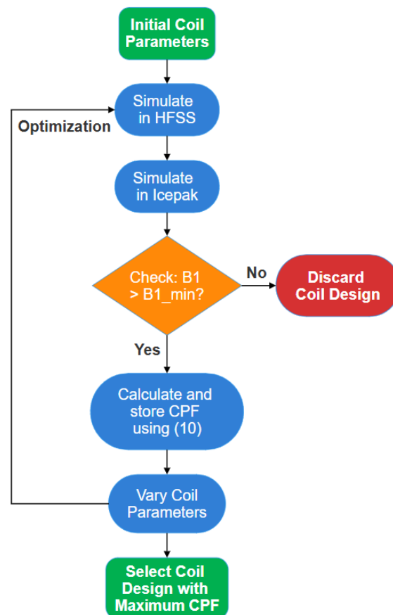
Figure 10. Optimization flowchart.
