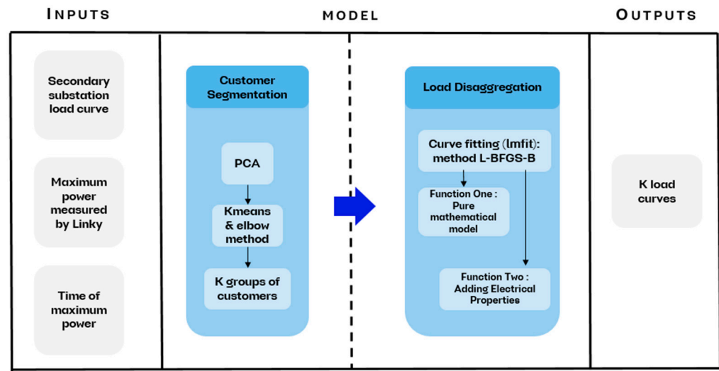
Figure 5. Schematic of the disaggregation model.
