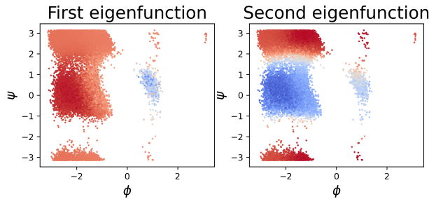
Figure 2: Two firsts non trivial eigenfunctions of the alanine dipeptide in water trained on a 250 ns simulation with \Delta t = 25 ps and displayed on an independant 250ns test simulation. The color of the points corresponds to the values of the eigenfunctions.
