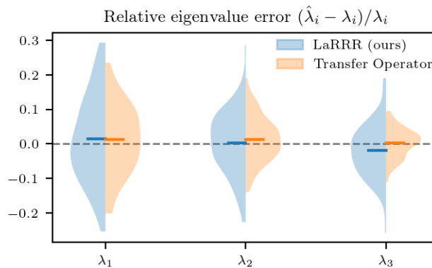
Figure 1: Relative error distributions for the leading eigenvalues \lambda_1 , \lambda_2 , and \lambda_3 of the generator and transfer operator, estimated from 100 independent trajectories of a 1D Langevin process on a triple-well potential. The relative errors are computed as (\hat{\lambda}_i - \lambda_i)/\lambda_i for each eigenvalue \lambda_i . The violin plots show the error distribution for both IG (blue) and TO (orange), with the thick bars the mean of the distribution.
