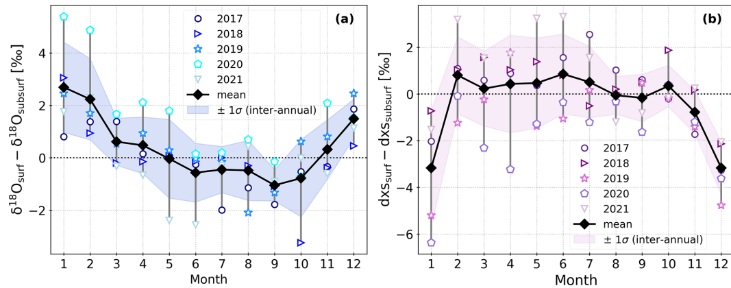
Figure 4. Mean annual cycle (monthly means) of the observed vertical difference between the snow surface and subsurface isotopic composition at Dome C. Panel (a) shows the mean annual cycle of the vertical difference in \delta^{18}\text{O} ; panel (b) shows the mean annual cycle of the vertical difference in d-excess. In both panels, the black diamonds correspond to the overall monthly means calculated over the 2017–2021 period. The shaded area shows the inter-annual variability in individual years around the overall monthly means (1 standard deviation), and the coloured markers show the monthly means for each individual year.
