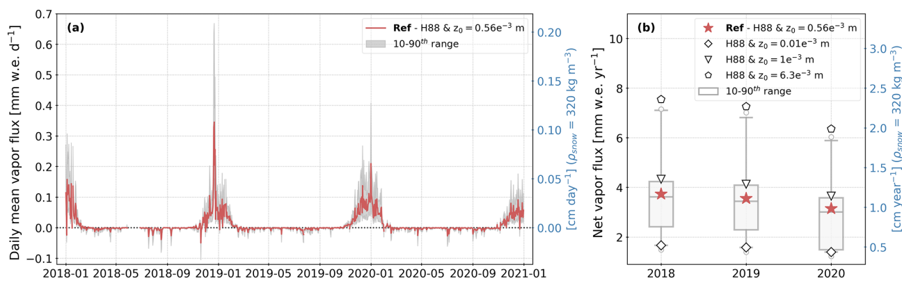
Figure 2. Water vapour flux at Dome C during the 2018–2020 period (positive for sublimation, negative for condensation). Panel (a) displays the 3-year time series of daily mean water vapour flux in millimetres of water equivalent. The red line corresponds to the reference parameterization, and the grey shading corresponds to the 10th–90th-percentile range of all parameterizations (described in Sect. 2.4.2). Panel (b) shows the net annual water vapour flux (sum of sublimation and condensation over 1 year). The red stars indicate the reference parameterization, and the three other black markers indicate the results using the stability function of H88 with a different z_0 . The whiskers of the grey boxplots indicate the 10th–90th-percentile range of all parameterizations, and the grey circles indicate the outliers outside of this range. The secondary axis to the right in blue gives water vapour fluxes in centimetres of snow, using a snow density ( \rho_{\text{snow}} = 320 \text{ kg m}^{-3} ) to convert SWE to snow height.
