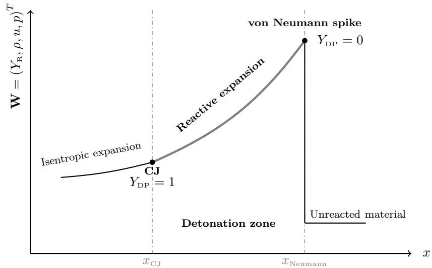
Figure 4: Schematic representation of a 1D detonation of an ideal explosive described by the ZND model. Mass transfer must be present only between the von Neumann spike and the CJ point when dealing with ideal explosives.
