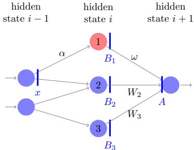
Fig. 2: Example of DAG Network. We assume a new node added in color red with new weights \alpha and \omega . We define pre-activities as A and post-activities as B or x.
