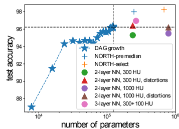
Fig. 4: Baselines on MNIST for test accuracy and number of parameters.
