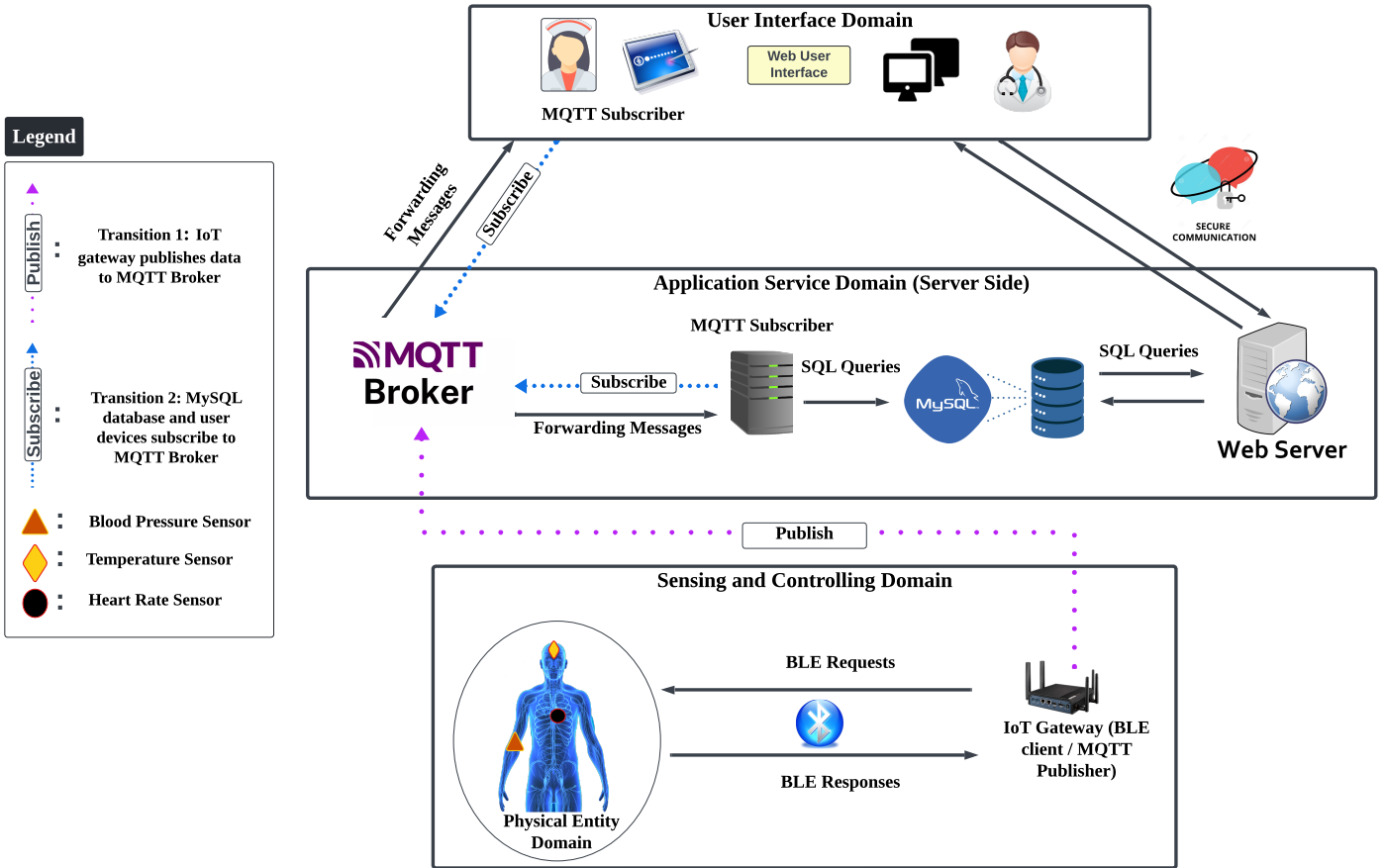
Figure 6: IoT Healthcare Application based on the ISO IoT Architecture
