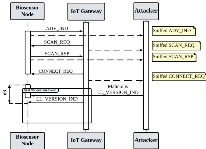
Figure 11: UML Sequence Diagram for the Attack Scenario Model Implementation 1.2 (ASMI-1.2).
