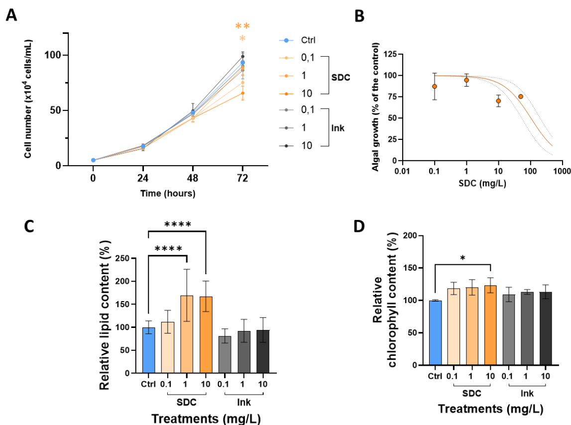
Figure 2: Effects of ink or SDC exposure towards the algae Raphidocelis subcapitata . A) Effects on the number of algal cells in culture over time when exposed to increasing concentrations of ink or SDC. B) Effects of 72h of an exposure to increasing concentrations of SDC on algal growth. C) Relative cellular content of neutral lipids expressed as percentage of the control group after 72h of exposure to different ink or SDC concentrations. D) Relative chlorophyll content expressed as percentage of the control in algae measured following 72h of exposure to different ink or SDC concentrations. Data are presented as mean \pm SD (n = 3 per condition). (ANOVA followed by Tukey. *: p < 0.05; **: p < 0.01 and ***: p < 0.001).
