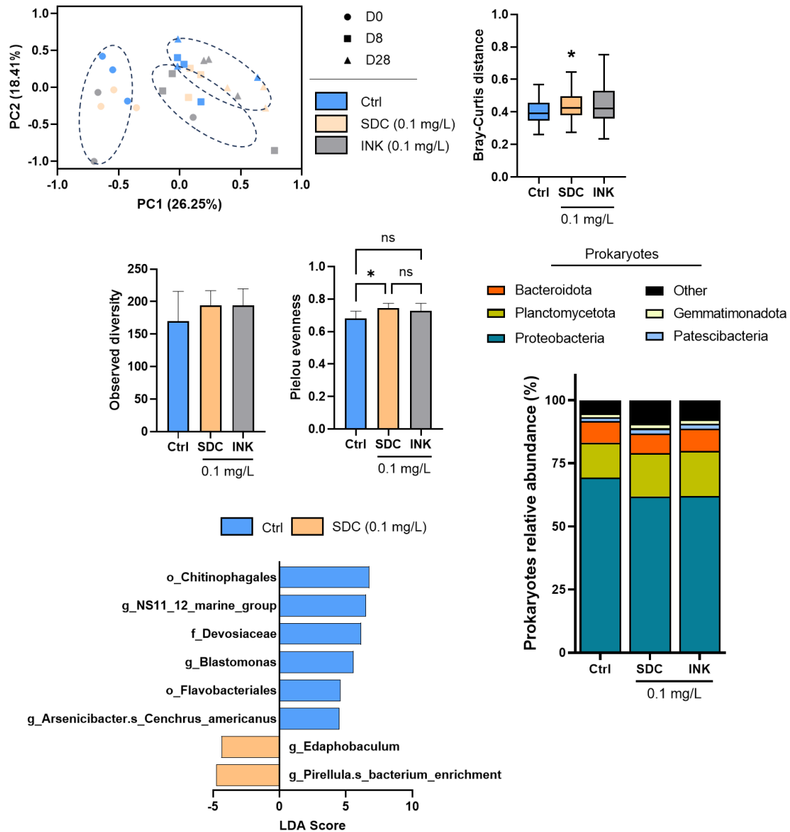
Figure 5: Effects of exposure to SDC and INK towards biofilm prokaryote communities. A) PCoA based on Bray-Curtis distances. B) Bray-Curtis distance. C) Observed diversity. D) Pielou evenness index. E) Relative abundances of the main phyla recovered in the biofilm. F) Taxa identified as differentially abundant between the control and the SDC-exposed group through LEfSe analysis. N = 9 samples per exposure condition (3 for each treatment duration). For alpha-diversity metrics and relative abundances of phyla, differences across groups were tested using ANOVA followed by Tukey's post-hoc test when p < 0.05 . Differences in Bray-
