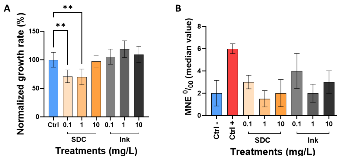
Figure 4: Effects of exposure to the commercial FLG-based ink or dispersant on X. laevis tadpoles. A) Effects on larvae normalized growth rate. Data are presented as mean \pm SD (n = 15 per condition). (ANOVA followed by Tukey. *: p<.05; **: p < 0.01 and ***: p < 0.001). B) Micronucleus induction measured in erythrocytes (MNE) in ‰. Data are presented as median \pm CI95% (n = 15 per condition). (McGill non-parametric test).
