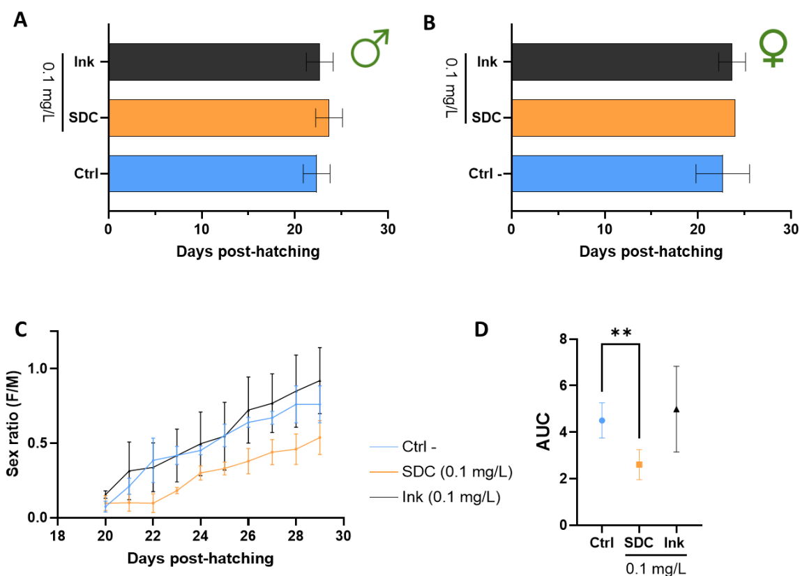
Figure 7: Effects of exposure to ink and SDC in C. riparius . A) Median day of emergence of adult males. B) Median day of emergence of adult females. C) Chironomid sex ratio over time (number of females / number of males). D) Area under the curve (AUC) calculated for the sex ratio over time. Data are presented as mean \pm SD (n = 3 per condition) (ANOVA followed by the Tukey test. *: p < 0.05; **: p < 0.01 and ***: p < 0.001).
