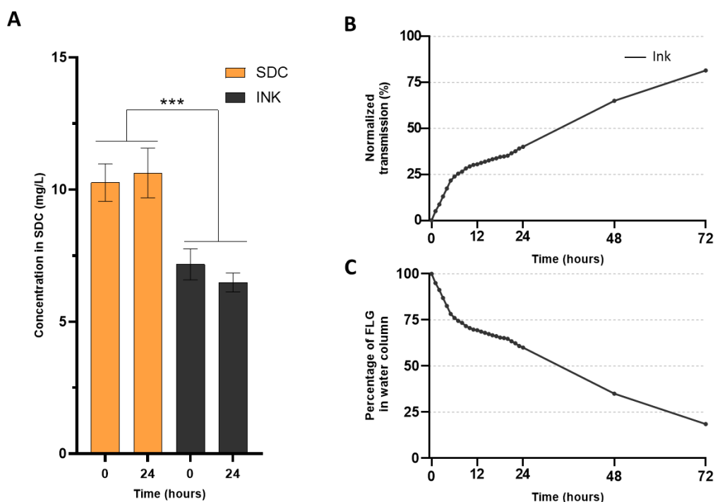
Figure 1: Characterization of ink and SDC behaviour in standardized exposure media (ISO, 2006). A) Effective concentrations of SDC (mg/L) in the water column measured in samples diluted to a nominal concentration of 10 mg/L of SDC solution alone and mixed with FLG to produce the ink at 0 and 24 h. B) Normalized transmission (%) in the water column over time in the presence of ink. C) Percentage of FLG from the ink in the water column over time. Data are presented as mean \pm SD ( n = 3 per condition). (ANOVA followed by Tukey. *: p < 0.05 ; **: p < 0.01 and ***: p < 0.001 ).
