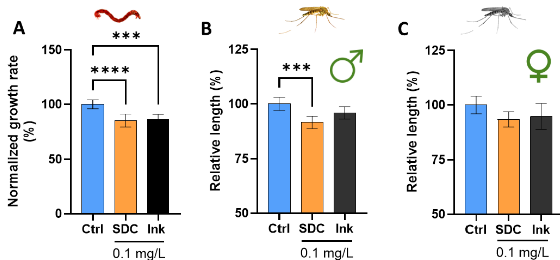
Figure 6: Effects of ink and SDC exposure in C. riparius with the normalized growth rate of 4-instar larvae after 8 days of exposure in % (A), the relative length of male adults in % (B) and the relative length of female adults in % (C). Data are presented as mean \pm SD ( n > 8 per condition). (ANOVA followed by Tukey. *: p < 0.05 ; **: p < 0.01 and ***: p < 0.001 ).
