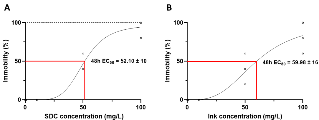
Figure 3: Percentage of Daphnia magna immobilization as a function of SDC concentration (A) and ink (B). Concentration response curves with 48h EC 50 calculated and presented as mean ± CI95% (n = 4 per condition).
